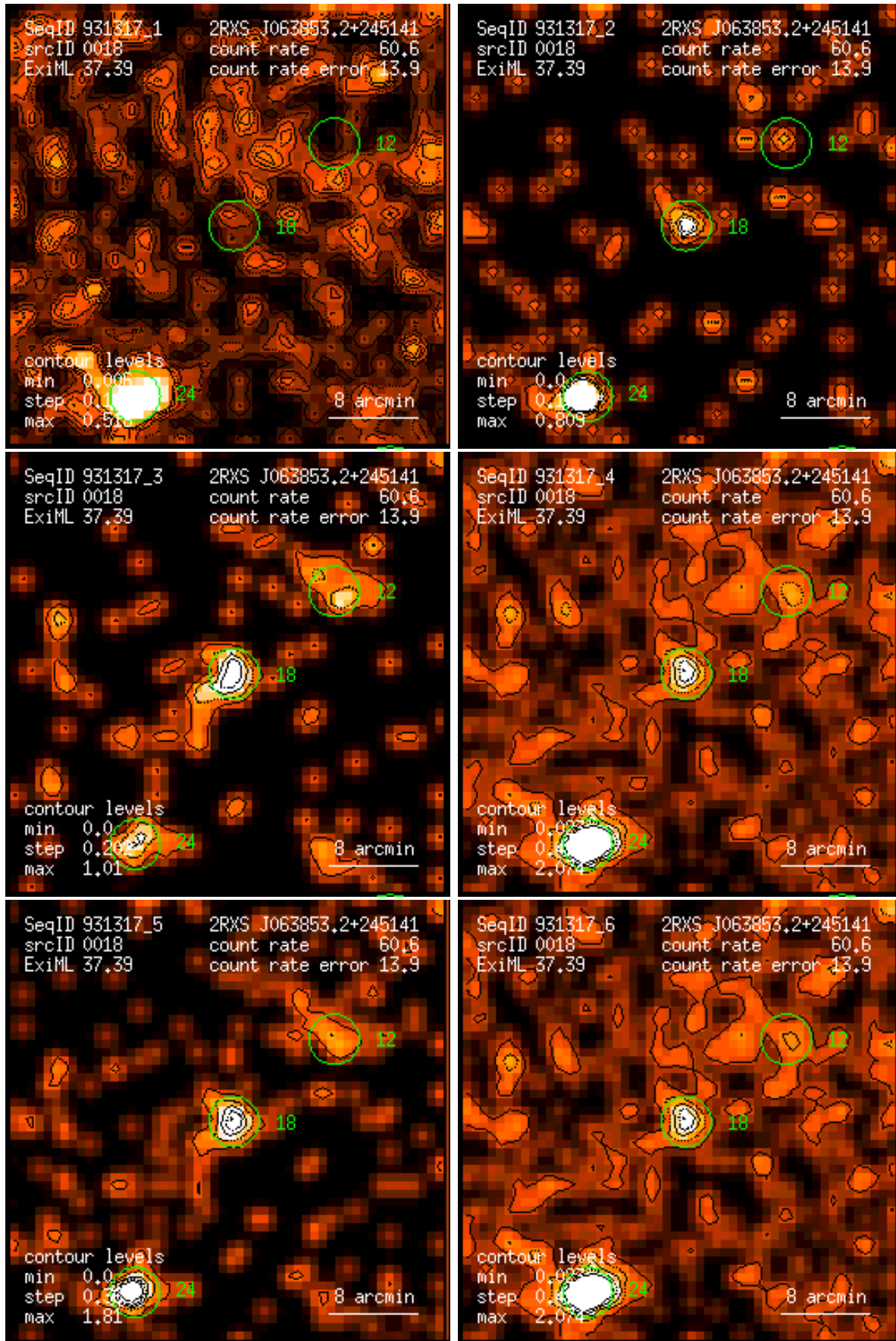
Figure 18: RASS 931317: detection 0018: band rate images, Gaussian filter: (1) PSPC channels 11 – 41, (2) 52 – 90, (3) 91 – 201, (4) 11 – 235, (5) 52 – 201, (6) 11 – 201. Broad band rates in counts/ks. Band rate contour levels in counts/ks/arcmin 2 .
