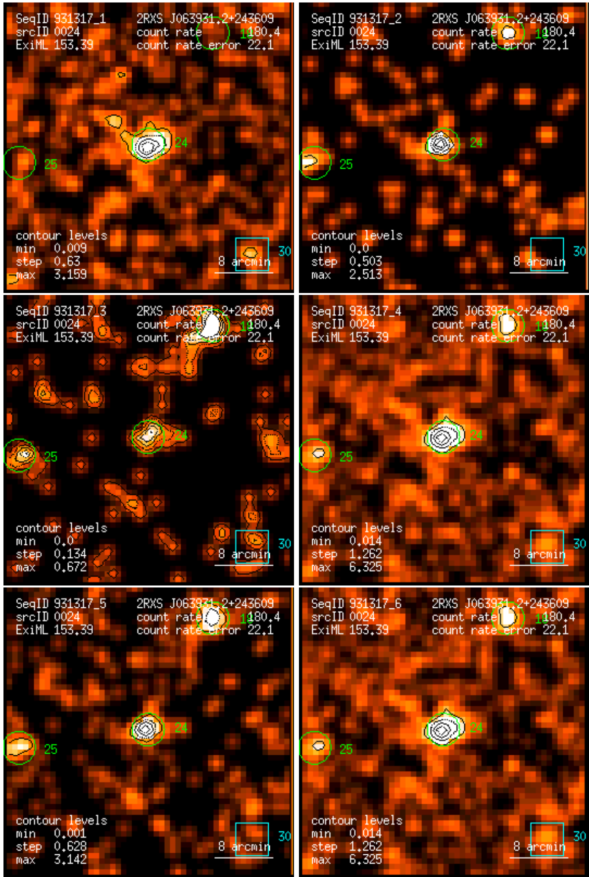
Figure 24: RASS 931317: detection 0024: band rate images, Gaussian filter: (1) PSPC channels 11 – 41, (2) 52 – 90, (3) 91 – 201, (4) 11 – 235, (5) 52 – 201, (6) 11 – 201. Broad band rates in counts/ks. Band rate contour levels in counts/ks/arcmin 2 .
