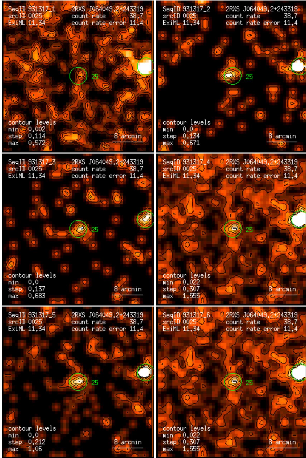
Figure 25: RASS 931317: detection 0025: band rate images, Gaussian filter: (1) PSPC channels 11 – 41, (2) 52 – 90, (3) 91 – 201, (4) 11 – 235, (5) 52 – 201, (6) 11 – 201. Broad band rates in counts/ks. Band rate contour levels in counts/ks/arcmin 2 .
