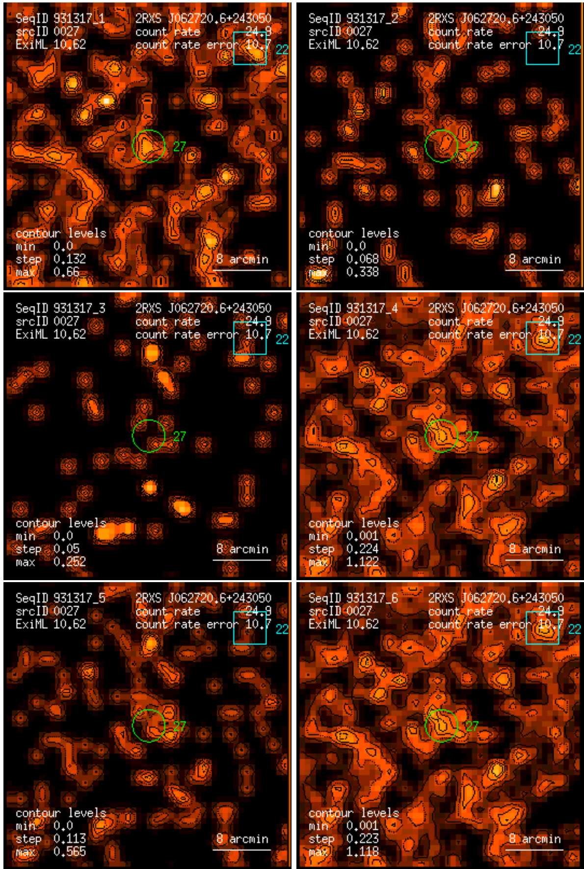
Figure 27: RASS 931317: detection 0027: band rate images, Gaussian filter: (1) PSPC channels 11 – 41, (2) 52 – 90, (3) 91 – 201, (4) 11 – 235, (5) 52 – 201, (6) 11 – 201. Broad band rates in counts/ks. Band rate contour levels in counts/ks/arcmin 2 .
