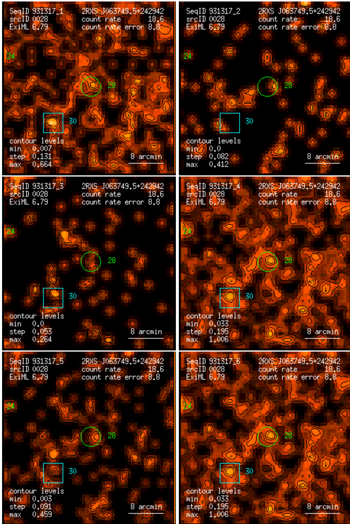
Figure 28: RASS 931317: detection 0028: band rate images, Gaussian filter: (1) PSPC channels 11 – 41, (2) 52 – 90, (3) 91 – 201, (4) 11 – 235, (5) 52 – 201, (6) 11 – 201. Broad band rates in counts/ks. Band rate contour levels in counts/ks/arcmin 2 .
