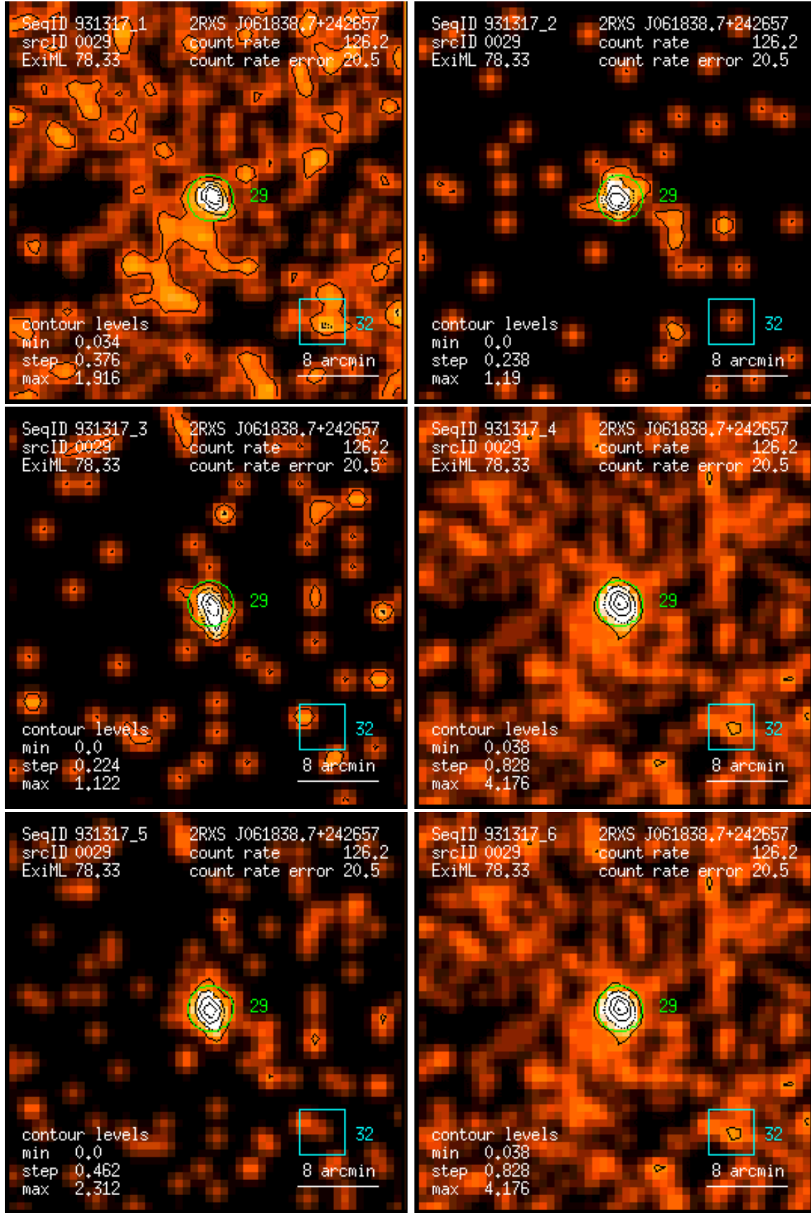
Figure 29: RASS 931317: detection 0029: band rate images, Gaussian filter: (1) PSPC channels 11 – 41, (2) 52 – 90, (3) 91 – 201, (4) 11 – 235, (5) 52 – 201, (6) 11 – 201. Broad band rates in counts/ks. Band rate contour levels in counts/ks/arcmin 2 .
