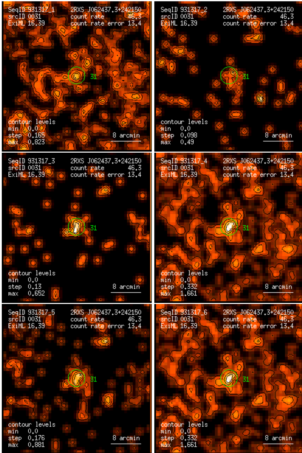
Figure 31: RASS 931317: detection 0031: band rate images, Gaussian filter: (1) PSPC channels 11 – 41, (2) 52 – 90, (3) 91 – 201, (4) 11 – 235, (5) 52 – 201, (6) 11 – 201. Broad band rates in counts/ks. Band rate contour levels in counts/ks/arcmin 2 .
