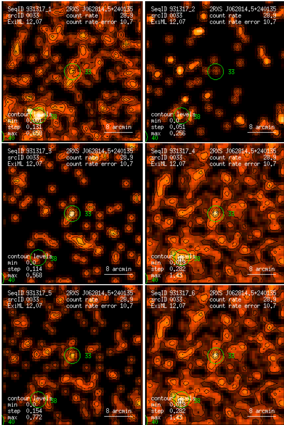
Figure 33: RASS 931317: detection 0033: band rate images, Gaussian filter: (1) PSPC channels 11 – 41, (2) 52 – 90, (3) 91 – 201, (4) 11 – 235, (5) 52 – 201, (6) 11 – 201. Broad band rates in counts/ks. Band rate contour levels in counts/ks/arcmin 2 .
