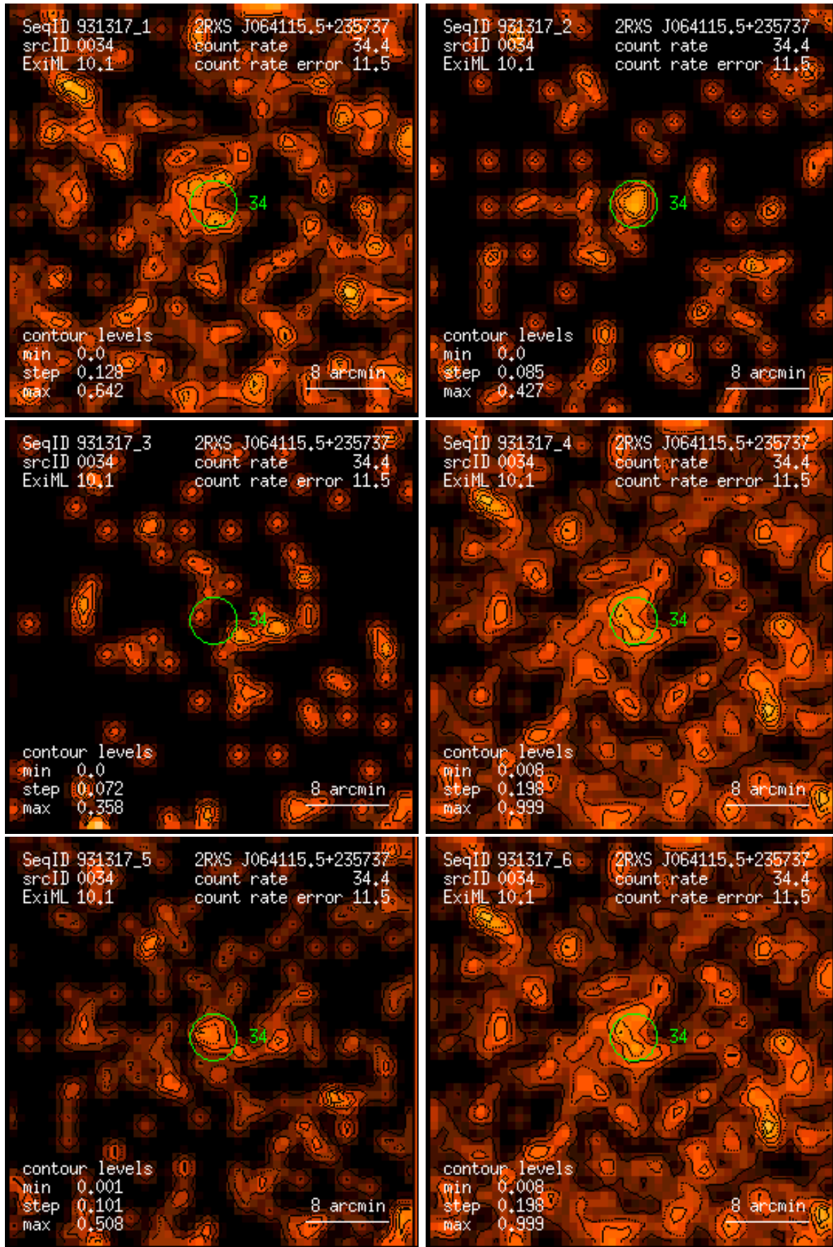
Figure 34: RASS 931317: detection 0034: band rate images, Gaussian filter: (1) PSPC channels 11 – 41, (2) 52 – 90, (3) 91 – 201, (4) 11 – 235, (5) 52 – 201, (6) 11 – 201. Broad band rates in counts/ks. Band rate contour levels in counts/ks/arcmin 2 .
