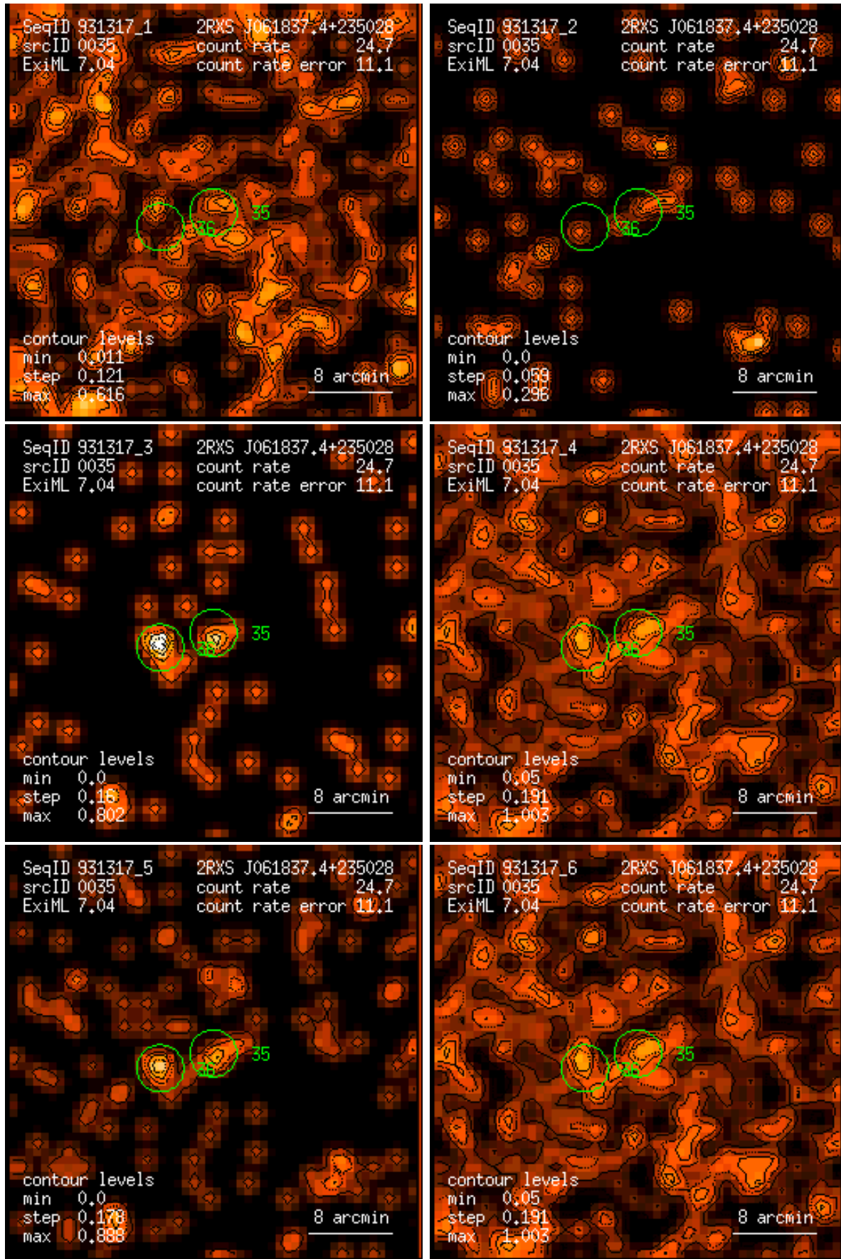
Figure 35: RASS 931317: detection 0035: band rate images, Gaussian filter: (1) PSPC channels 11 – 41, (2) 52 – 90, (3) 91 – 201, (4) 11 – 235, (5) 52 – 201, (6) 11 – 201. Broad band rates in counts/ks. Band rate contour levels in counts/ks/arcmin 2 .
