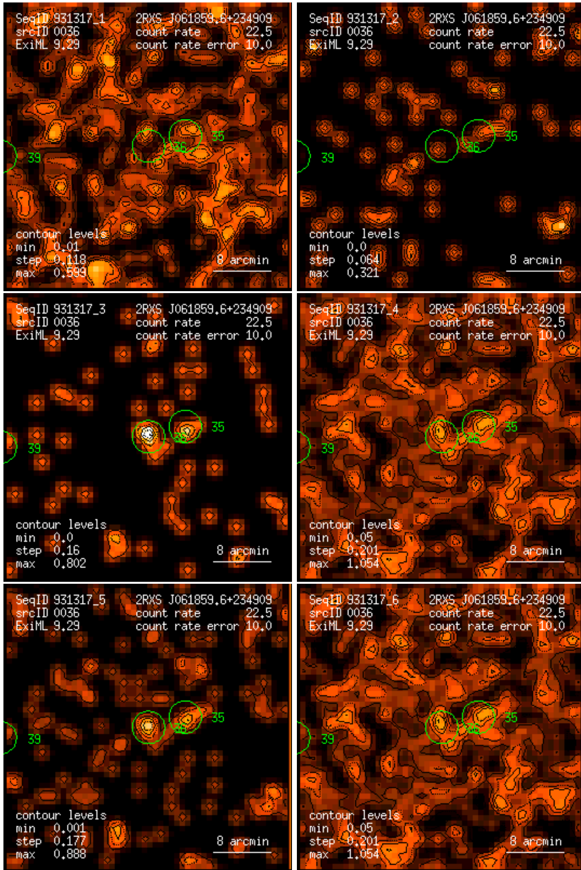
Figure 36: RASS 931317: detection 0036: band rate images, Gaussian filter: (1) PSPC channels 11 – 41, (2) 52 – 90, (3) 91 – 201, (4) 11 – 235, (5) 52 – 201, (6) 11 – 201. Broad band rates in counts/ks. Band rate contour levels in counts/ks/arcmin 2 .
