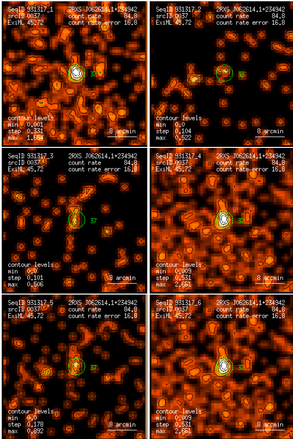
Figure 37: RASS 931317: detection 0037: band rate images, Gaussian filter: (1) PSPC channels 11 – 41, (2) 52 – 90, (3) 91 – 201, (4) 11 – 235, (5) 52 – 201, (6) 11 – 201. Broad band rates in counts/ks. Band rate contour levels in counts/ks/arcmin 2 .
