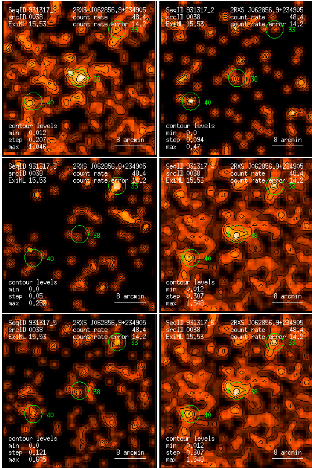
Figure 38: RASS 931317: detection 0038: band rate images, Gaussian filter: (1) PSPC channels 11 – 41, (2) 52 – 90, (3) 91 – 201, (4) 11 – 235, (5) 52 – 201, (6) 11 – 201. Broad band rates in counts/ks. Band rate contour levels in counts/ks/arcmin 2 .
