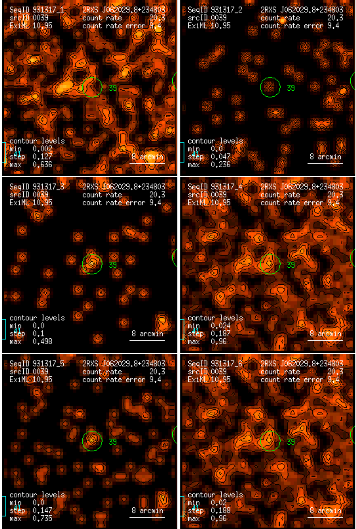
Figure 39: RASS 931317: detection 0039: band rate images, Gaussian filter: (1) PSPC channels 11 – 41, (2) 52 – 90, (3) 91 – 201, (4) 11 – 235, (5) 52 – 201, (6) 11 – 201. Broad band rates in counts/ks. Band rate contour levels in counts/ks/arcmin 2 .
