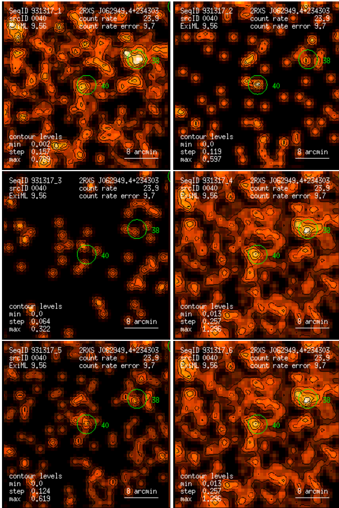
Figure 40: RASS 931317: detection 0040: band rate images, Gaussian filter: (1) PSPC channels 11 – 41, (2) 52 – 90, (3) 91 – 201, (4) 11 – 235, (5) 52 – 201, (6) 11 – 201. Broad band rates in counts/ks. Band rate contour levels in counts/ks/arcmin 2 .
