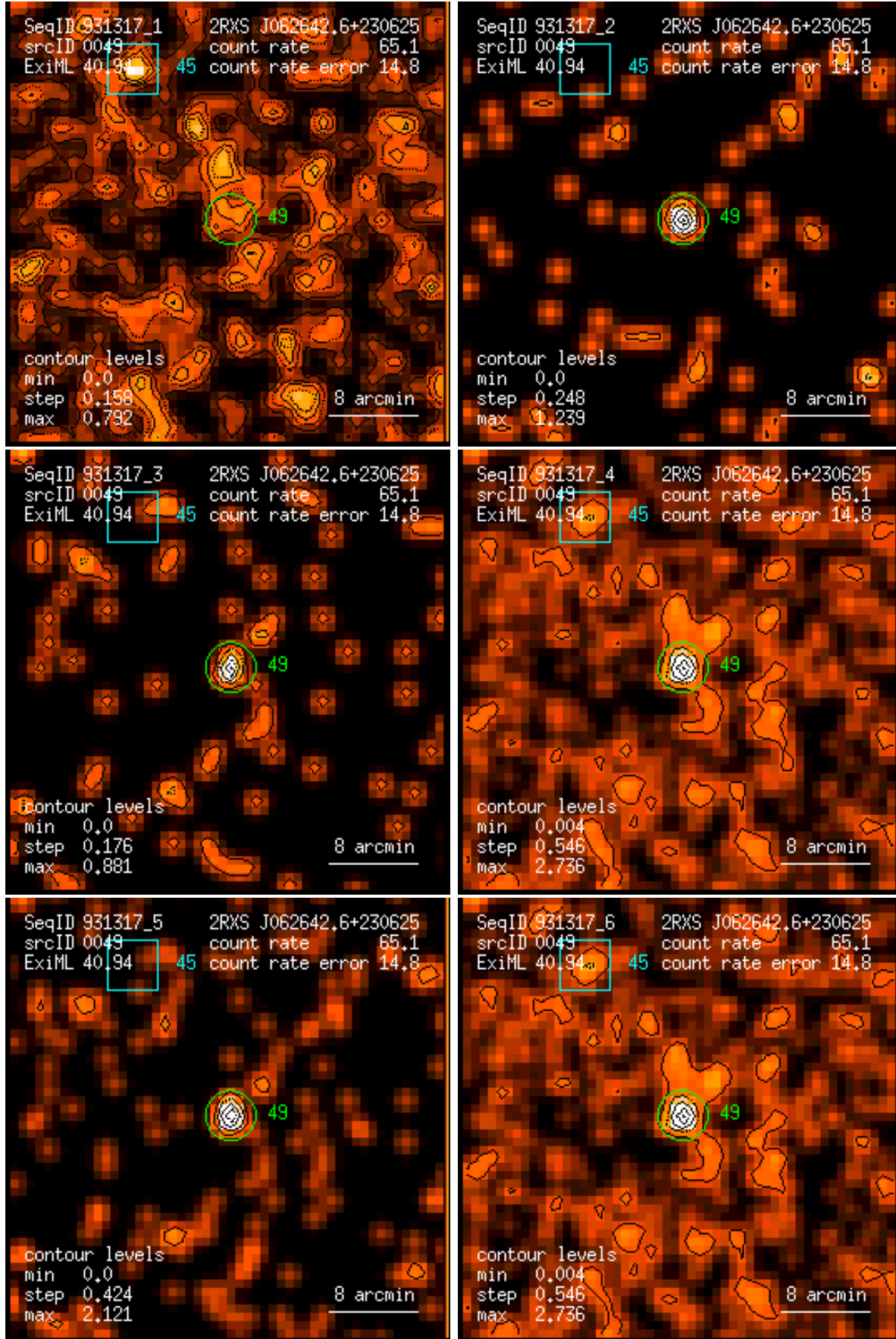
Figure 49: RASS 931317: detection 0049: band rate images, Gaussian filter: (1) PSPC channels 11 – 41, (2) 52 – 90, (3) 91 – 201, (4) 11 – 235, (5) 52 – 201, (6) 11 – 201. Broad band rates in counts/ks. Band rate contour levels in counts/ks/arcmin 2 .
