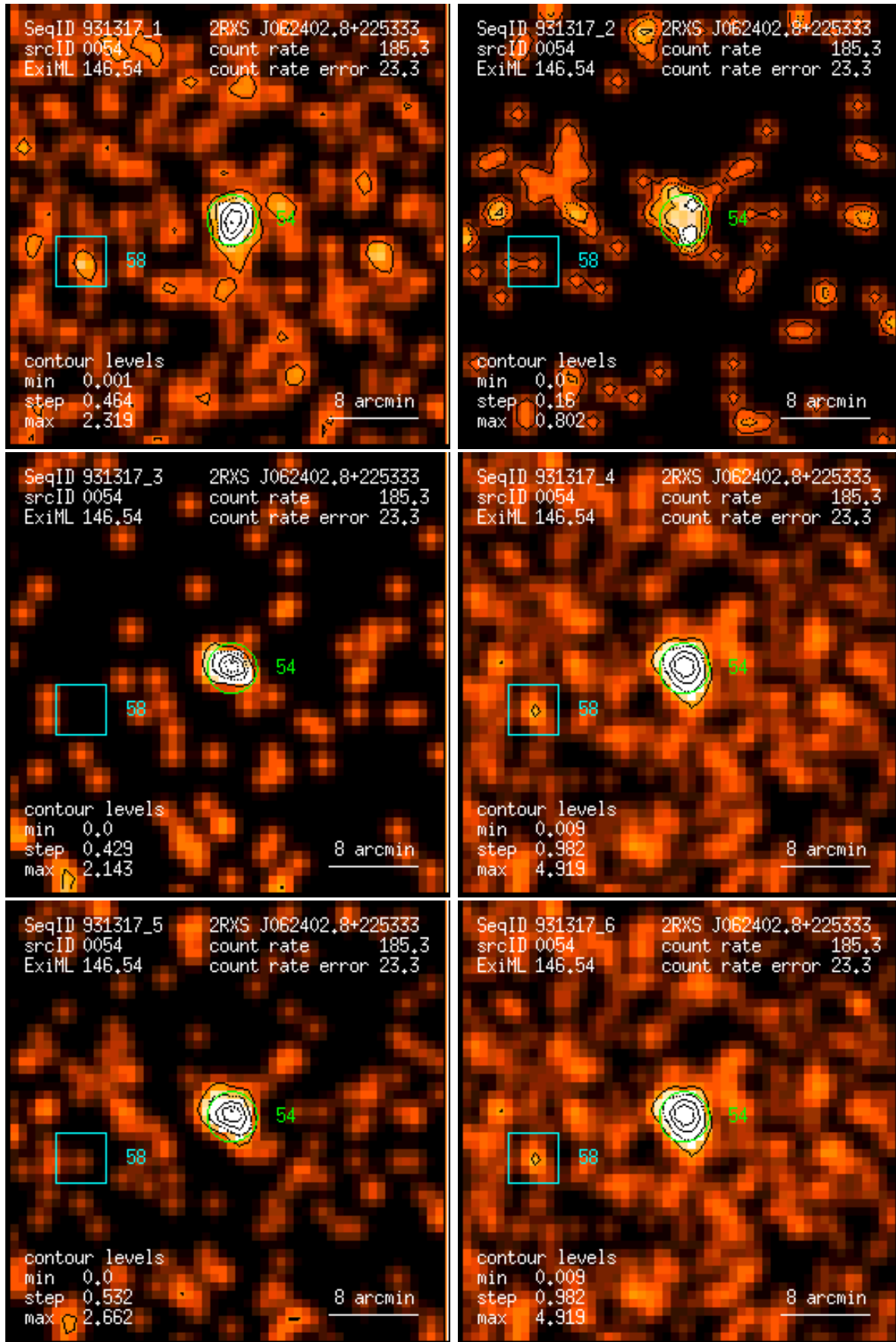
Figure 54: RASS 931317: detection 0054: band rate images, Gaussian filter: (1) PSPC channels 11 – 41, (2) 52 – 90, (3) 91 – 201, (4) 11 – 235, (5) 52 – 201, (6) 11 – 201. Broad band rates in counts/ks. Band rate contour levels in counts/ks/arcmin 2 .
