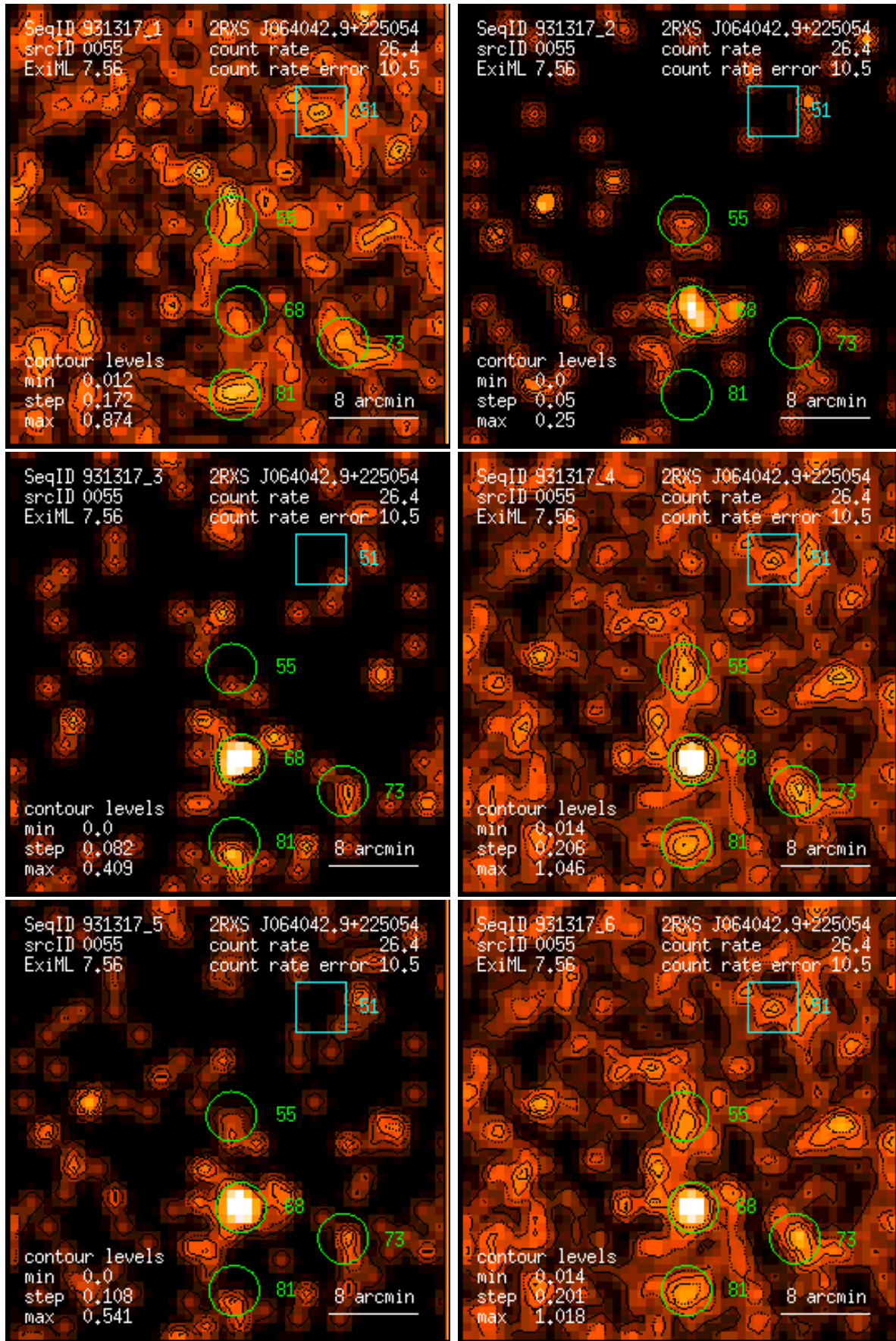
Figure 55: RASS 931317: detection 0055: band rate images, Gaussian filter: (1) PSPC channels 11 – 41, (2) 52 – 90, (3) 91 – 201, (4) 11 – 235, (5) 52 – 201, (6) 11 – 201. Broad band rates in counts/ks. Band rate contour levels in counts/ks/arcmin 2 .
