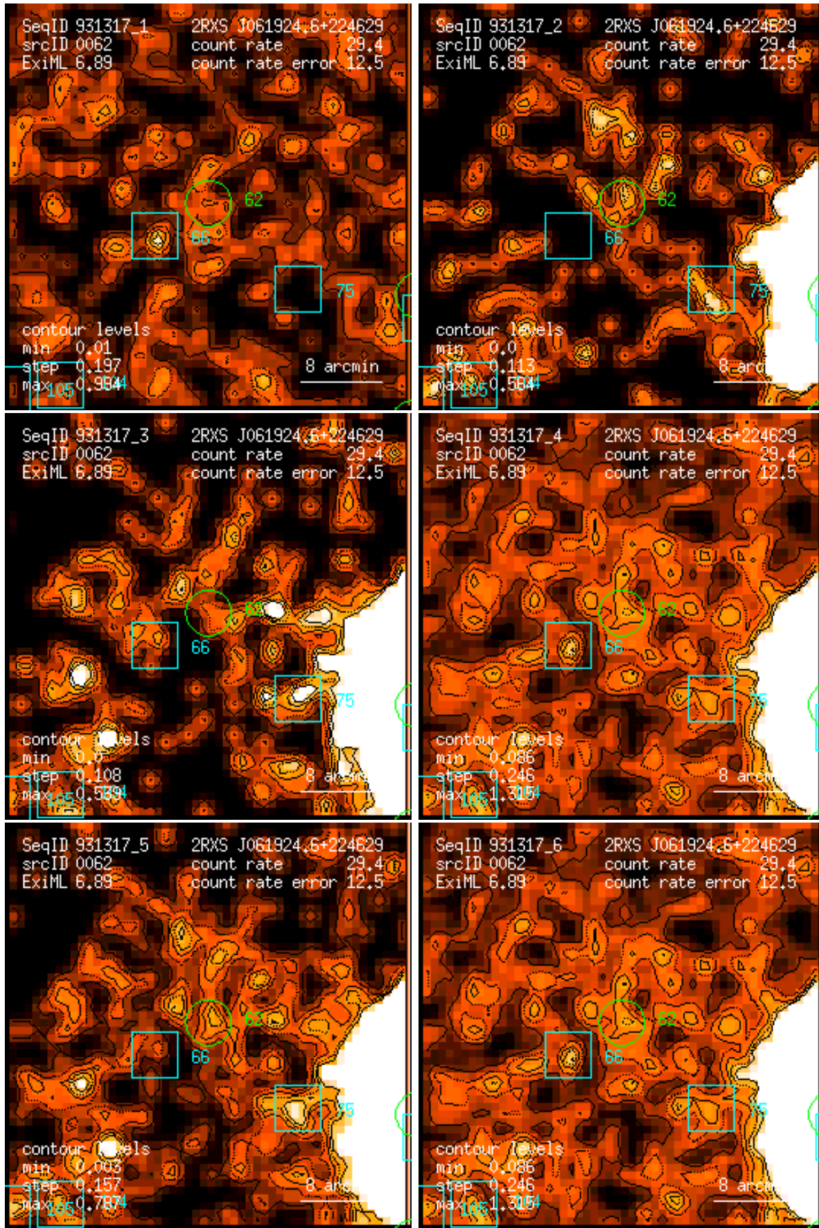
Figure 62: RASS 931317: detection 0062: band rate images, Gaussian filter: (1) PSPC channels 11 – 41, (2) 52 – 90, (3) 91 – 201, (4) 11 – 235, (5) 52 – 201, (6) 11 – 201. Broad band rates in counts/ks. Band rate contour levels in counts/ks/arcmin 2 .
