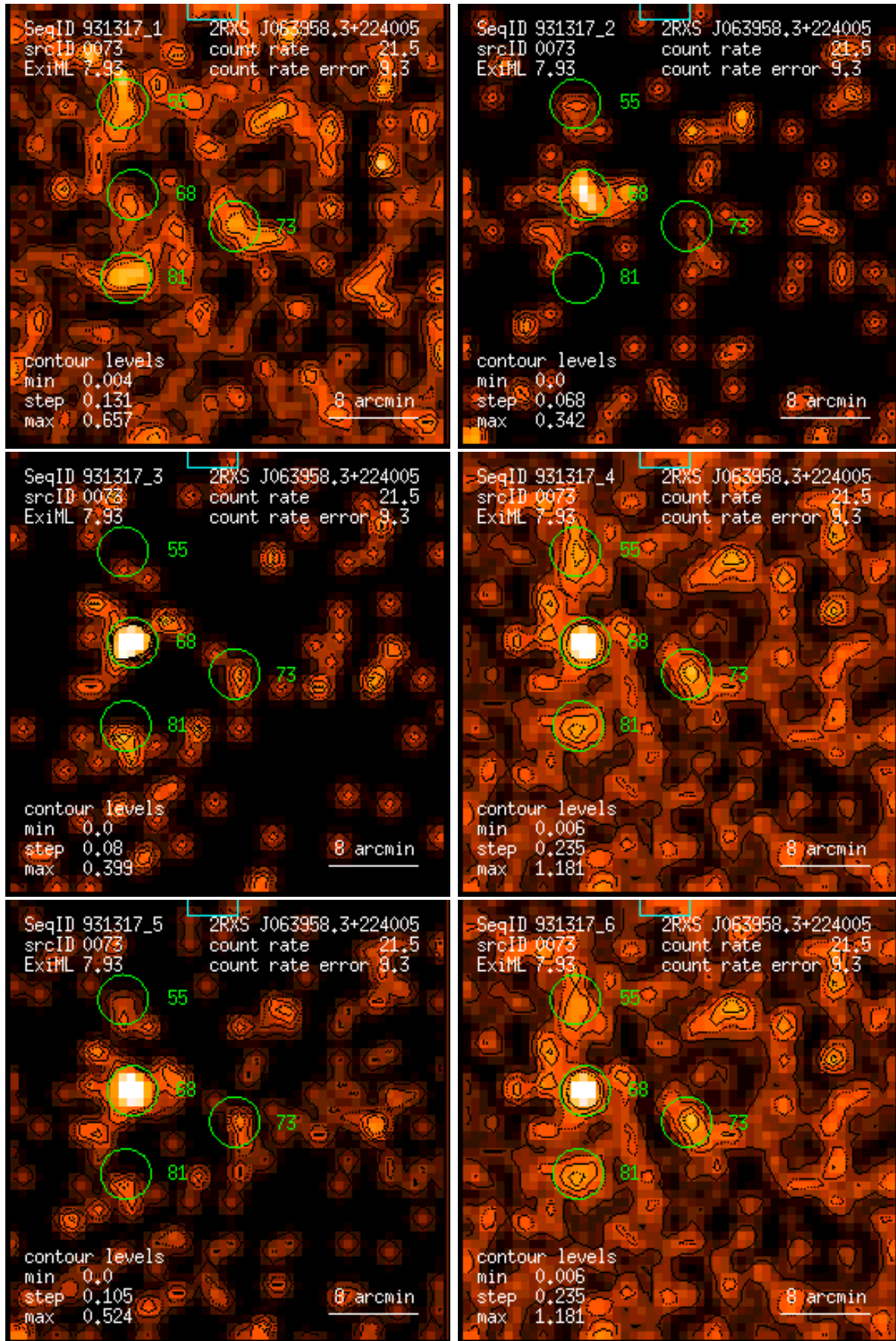
Figure 73: RASS 931317: detection 0073: band rate images, Gaussian filter: (1) PSPC channels 11 – 41, (2) 52 – 90, (3) 91 – 201, (4) 11 – 235, (5) 52 – 201, (6) 11 – 201. Broad band rates in counts/ks. Band rate contour levels in counts/ks/arcmin 2 .
