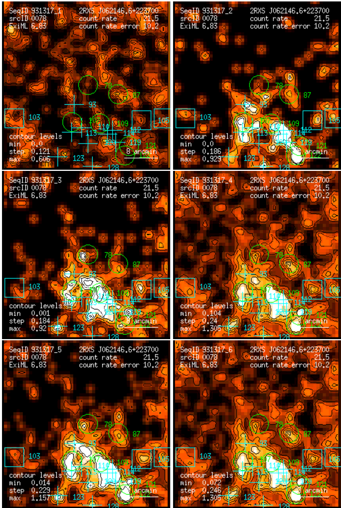
Figure 78: RASS 931317: detection 0078: band rate images, Gaussian filter: (1) PSPC channels 11 – 41, (2) 52 – 90, (3) 91 – 201, (4) 11 – 235, (5) 52 – 201, (6) 11 – 201. Broad band rates in counts/ks. Band rate contour levels in counts/ks/arcmin 2 .
