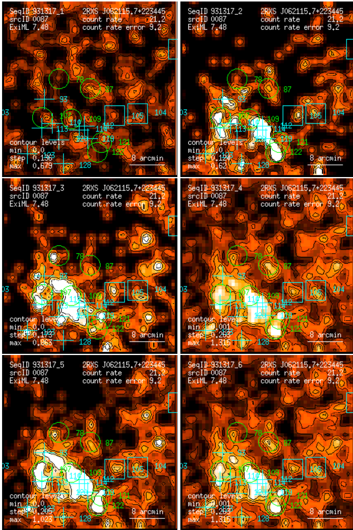
Figure 87: RASS 931317: detection 0087: band rate images, Gaussian filter: (1) PSPC channels 11 – 41, (2) 52 – 90, (3) 91 – 201, (4) 11 – 235, (5) 52 – 201, (6) 11 – 201. Broad band rates in counts/ks. Band rate contour levels in counts/ks/arcmin 2 .
