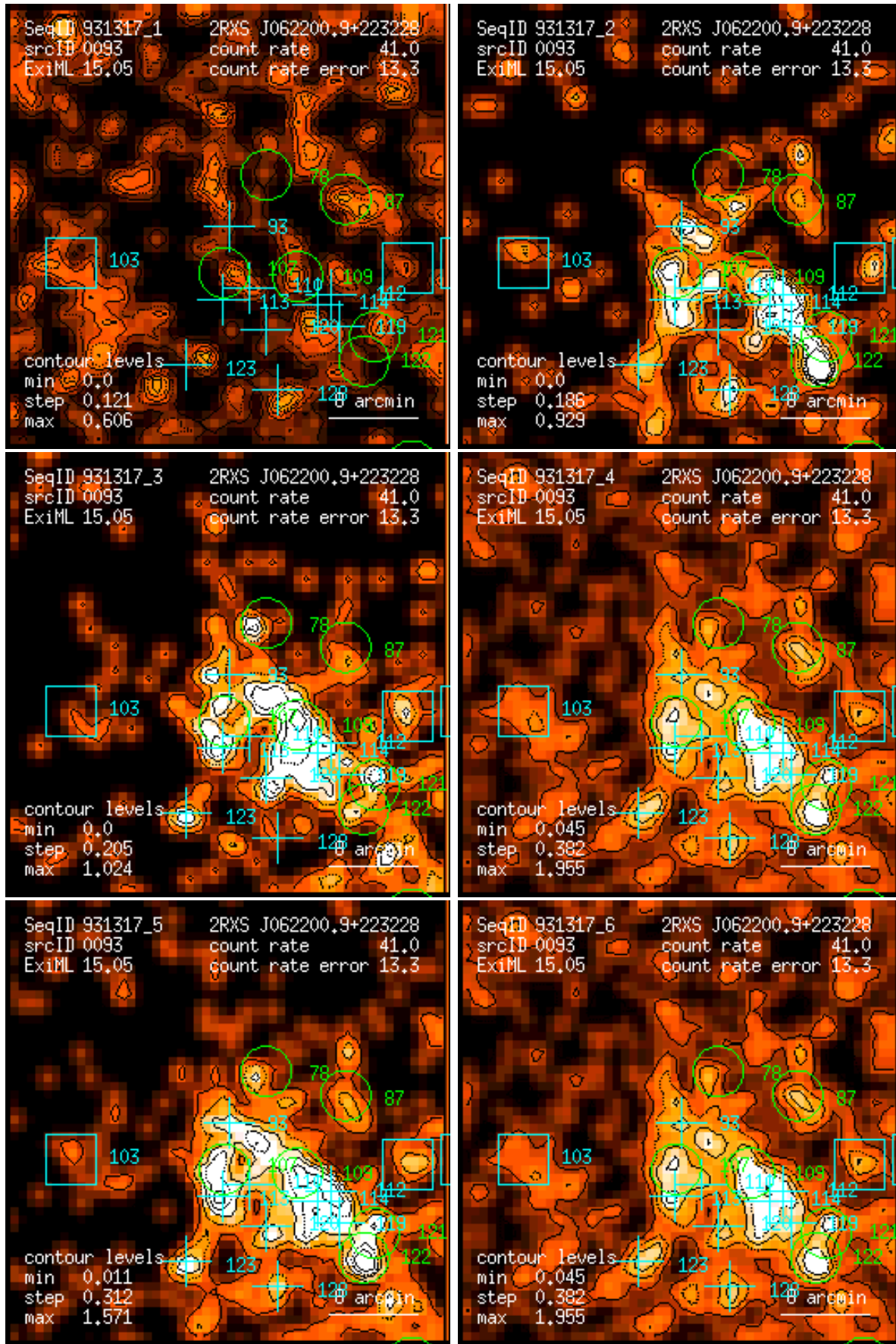
Figure 93: RASS 931317: detection 0093: band rate images, Gaussian filter: (1) PSPC channels 11 – 41, (2) 52 – 90, (3) 91 – 201, (4) 11 – 235, (5) 52 – 201, (6) 11 – 201. Broad band rates in counts/ks. Band rate contour levels in counts/ks/arcmin 2 .
