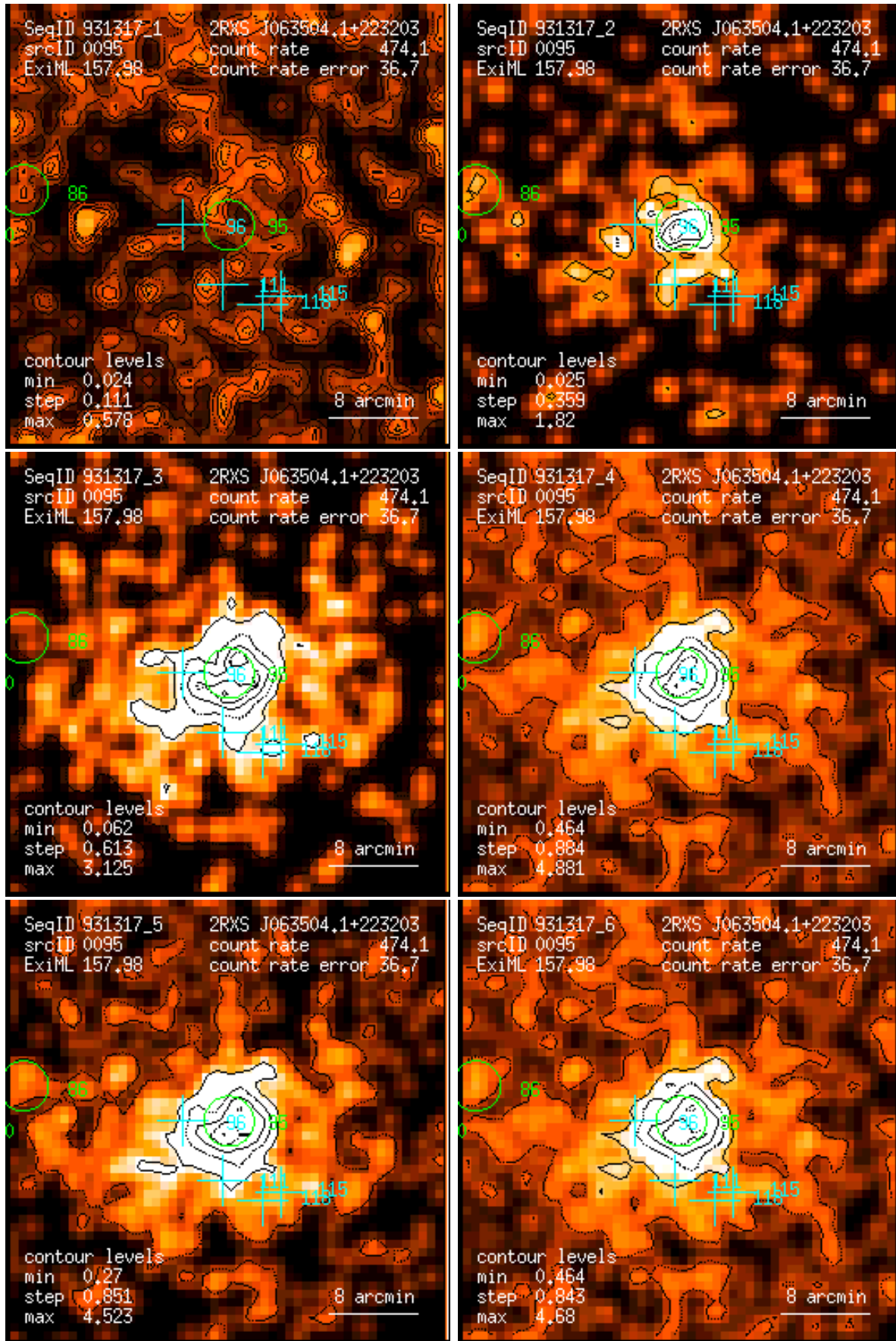
Figure 95: RASS 931317: detection 0095: band rate images, Gaussian filter: (1) PSPC channels 11 – 41, (2) 52 – 90, (3) 91 – 201, (4) 11 – 235, (5) 52 – 201, (6) 11 – 201. Broad band rates in counts/ks. Band rate contour levels in counts/ks/arcmin 2 .
