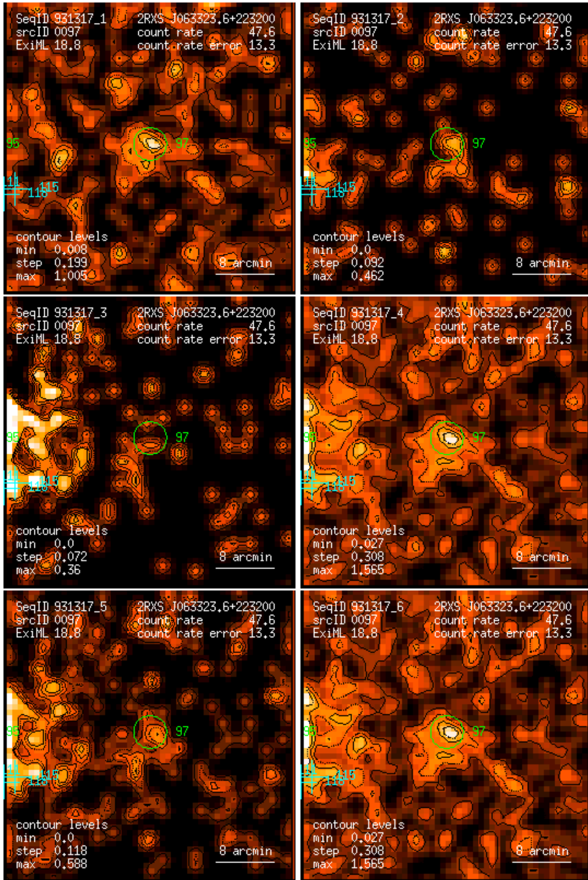
Figure 97: RASS 931317: detection 0097: band rate images, Gaussian filter: (1) PSPC channels 11 – 41, (2) 52 – 90, (3) 91 – 201, (4) 11 – 235, (5) 52 – 201, (6) 11 – 201. Broad band rates in counts/ks. Band rate contour levels in counts/ks/arcmin 2 .
