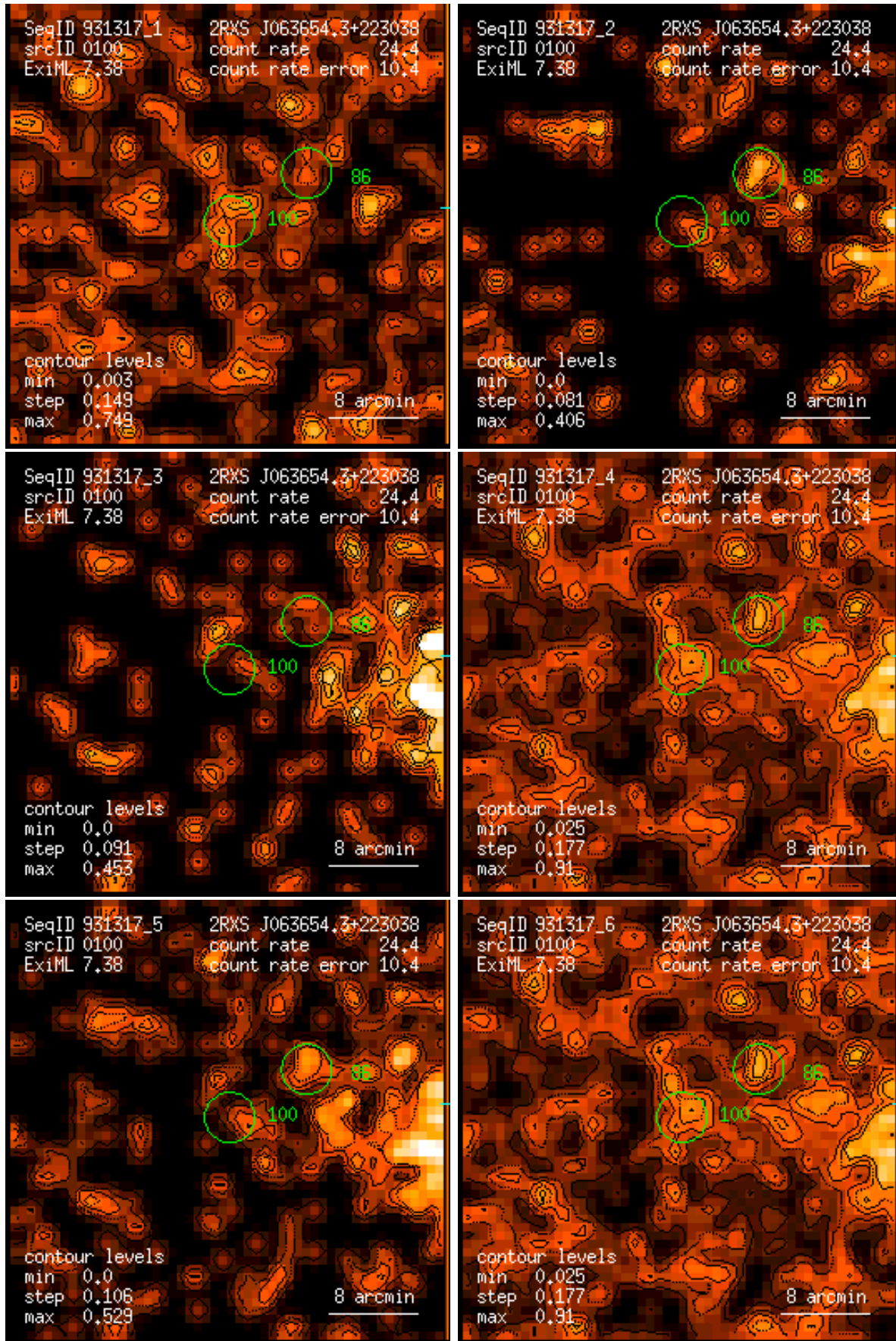
Figure 100: RASS 931317: detection 0100: band rate images, Gaussian filter: (1) PSPC channels 11 – 41, (2) 52 – 90, (3) 91 – 201, (4) 11 – 235, (5) 52 – 201, (6) 11 – 201. Broad band rates in counts/ks. Band rate contour levels in counts/ks/arcmin 2 .
