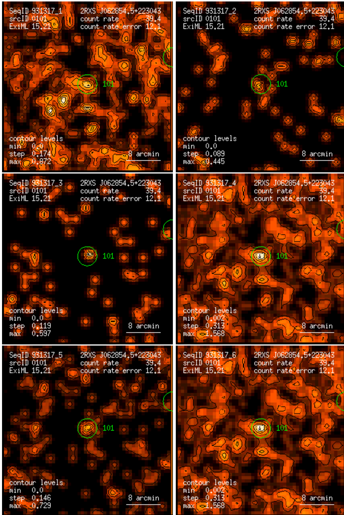
Figure 101: RASS 931317: detection 0101: band rate images, Gaussian filter: (1) PSPC channels 11 – 41, (2) 52 – 90, (3) 91 – 201, (4) 11 – 235, (5) 52 – 201, (6) 11 – 201. Broad band rates in counts/ks. Band rate contour levels in counts/ks/arcmin 2 .
