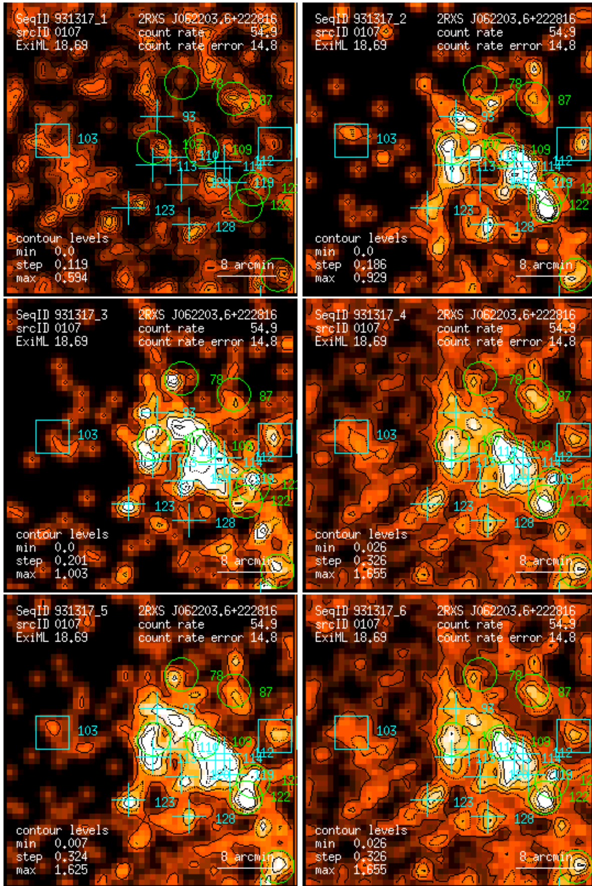
Figure 107: RASS 931317: detection 0107: band rate images, Gaussian filter: (1) PSPC channels 11 – 41, (2) 52 – 90, (3) 91 – 201, (4) 11 – 235, (5) 52 – 201, (6) 11 – 201. Broad band rates in counts/ks. Band rate contour levels in counts/ks/arcmin 2 .
