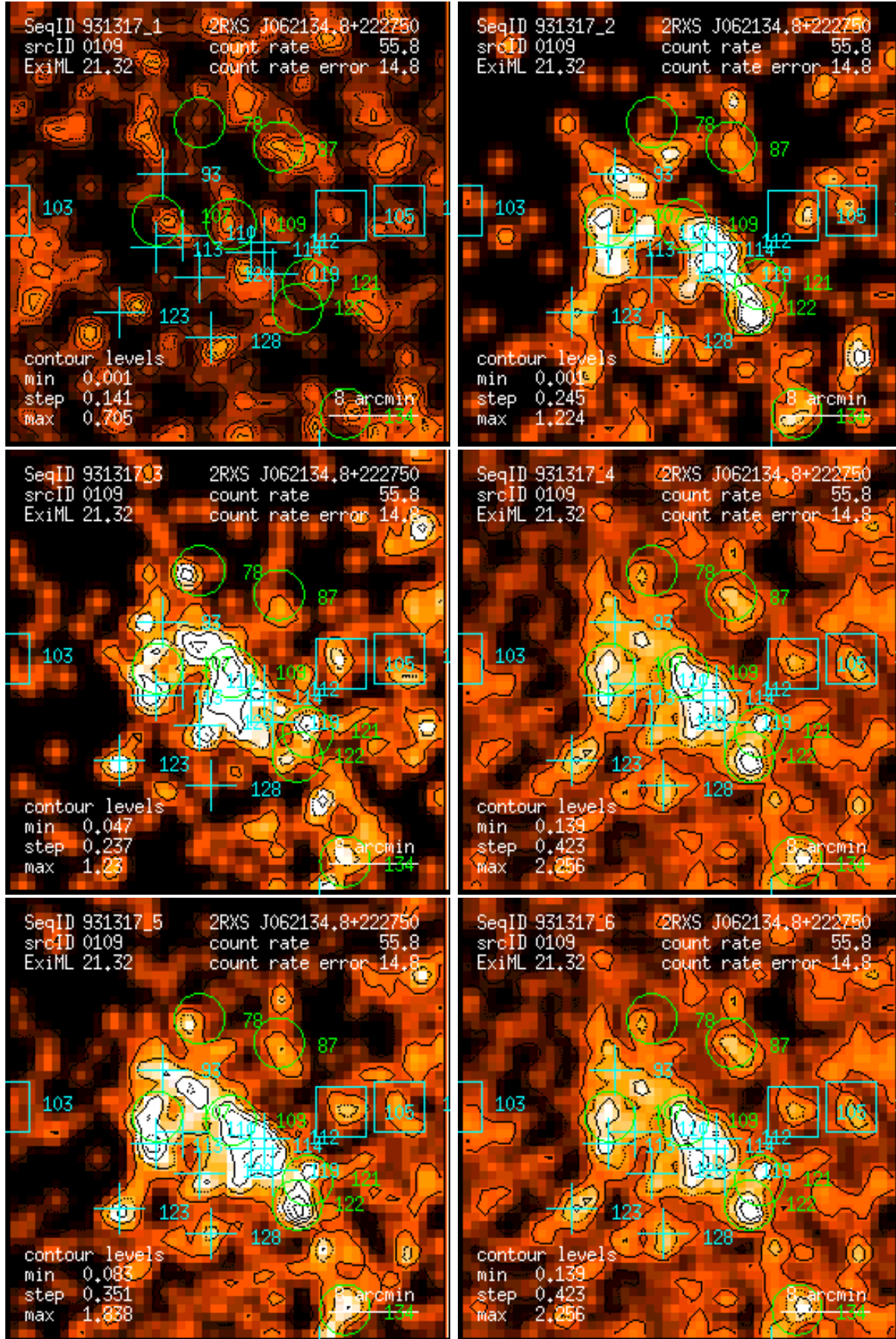
Figure 109: RASS 931317: detection 0109: band rate images, Gaussian filter: (1) PSPC channels 11 – 41, (2) 52 – 90, (3) 91 – 201, (4) 11 – 235, (5) 52 – 201, (6) 11 – 201. Broad band rates in counts/ks. Band rate contour levels in counts/ks/arcmin 2 .
