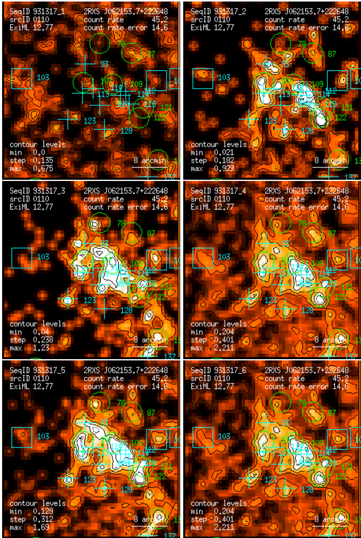
Figure 110: RASS 931317: detection 0110: band rate images, Gaussian filter: (1) PSPC channels 11 – 41, (2) 52 – 90, (3) 91 – 201, (4) 11 – 235, (5) 52 – 201, (6) 11 – 201. Broad band rates in counts/ks. Band rate contour levels in counts/ks/arcmin 2 .
