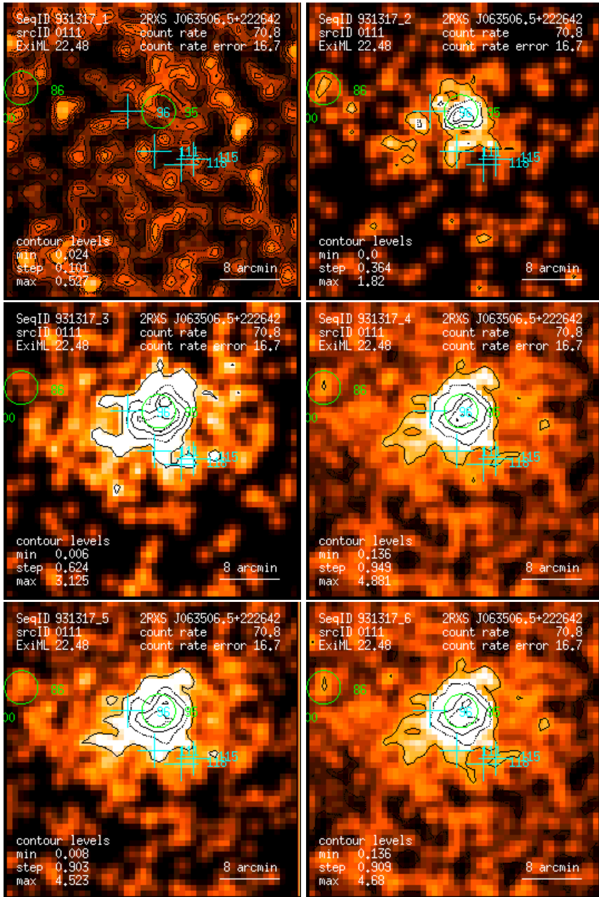
Figure 111: RASS 931317: detection 0111: band rate images, Gaussian filter: (1) PSPC channels 11 – 41, (2) 52 – 90, (3) 91 – 201, (4) 11 – 235, (5) 52 – 201, (6) 11 – 201. Broad band rates in counts/ks. Band rate contour levels in counts/ks/arcmin 2 .
