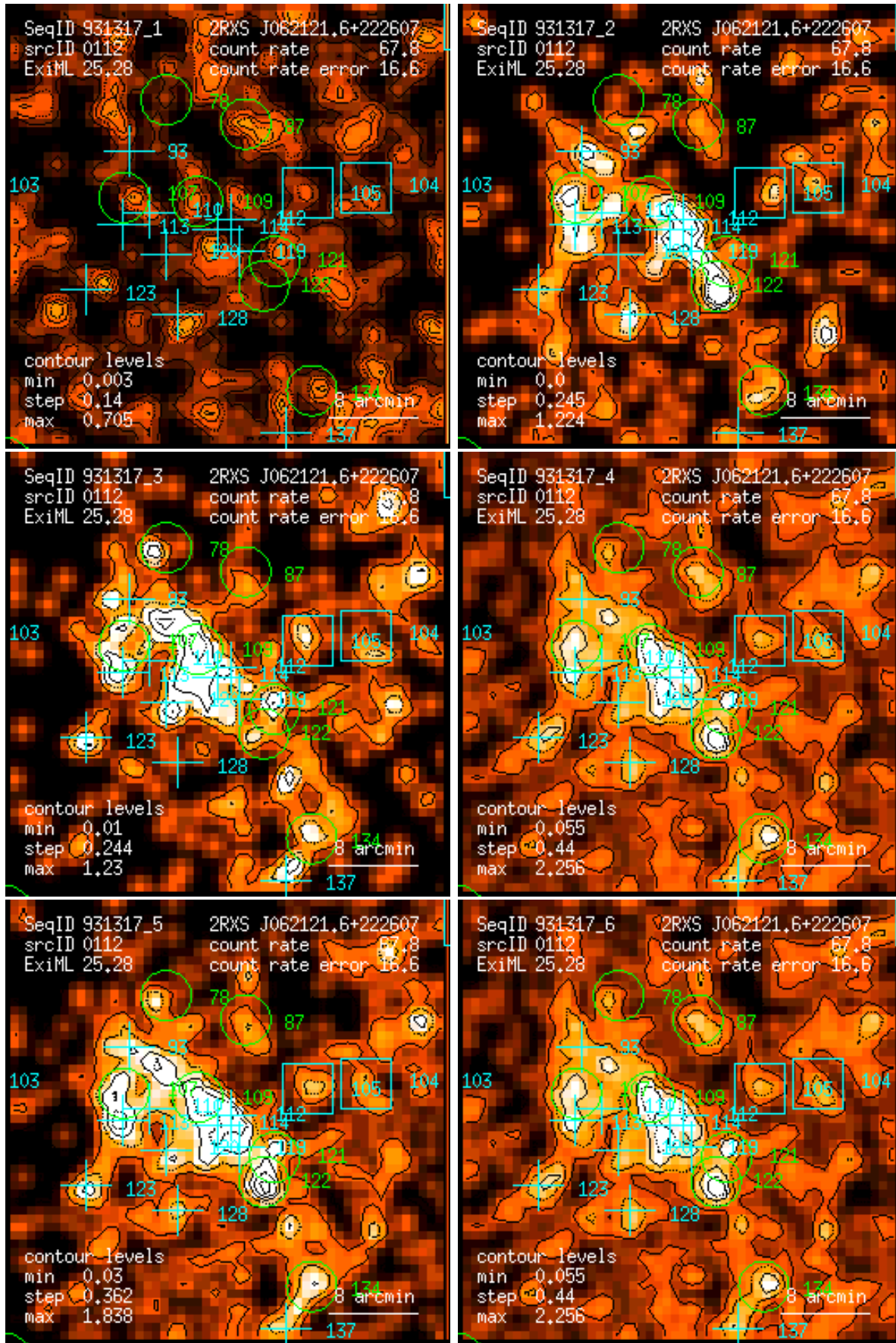
Figure 112: RASS 931317: detection 0112: band rate images, Gaussian filter: (1) PSPC channels 11 – 41, (2) 52 – 90, (3) 91 – 201, (4) 11 – 235, (5) 52 – 201, (6) 11 – 201. Broad band rates in counts/ks. Band rate contour levels in counts/ks/arcmin 2 .
