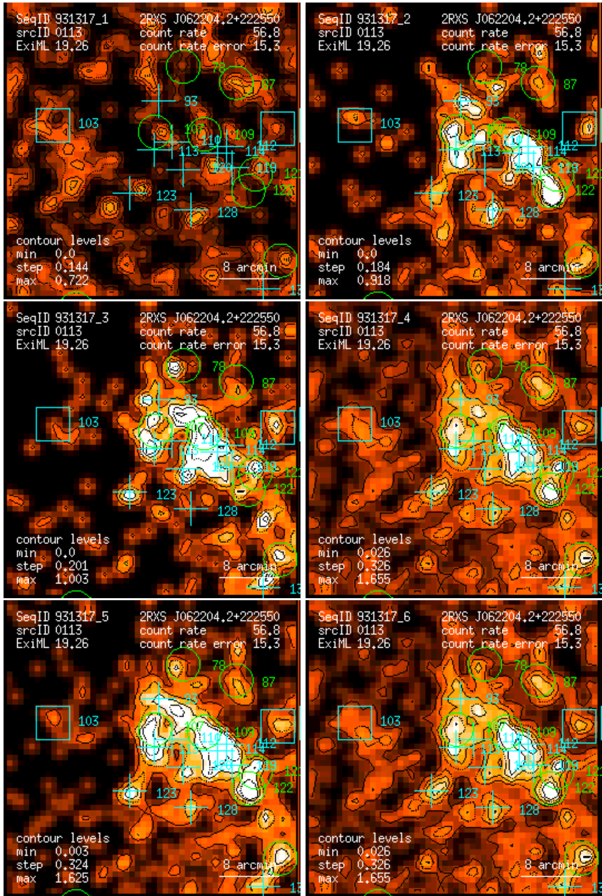
Figure 113: RASS 931317: detection 0113: band rate images, Gaussian filter: (1) PSPC channels 11 – 41, (2) 52 – 90, (3) 91 – 201, (4) 11 – 235, (5) 52 – 201, (6) 11 – 201. Broad band rates in counts/ks. Band rate contour levels in counts/ks/arcmin 2 .
