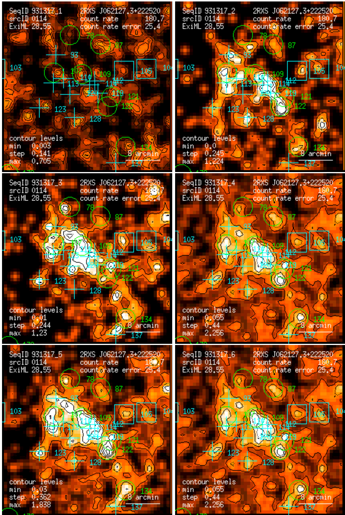
Figure 114: RASS 931317: detection 0114: band rate images, Gaussian filter: (1) PSPC channels 11 – 41, (2) 52 – 90, (3) 91 – 201, (4) 11 – 235, (5) 52 – 201, (6) 11 – 201. Broad band rates in counts/ks. Band rate contour levels in counts/ks/arcmin 2 .
