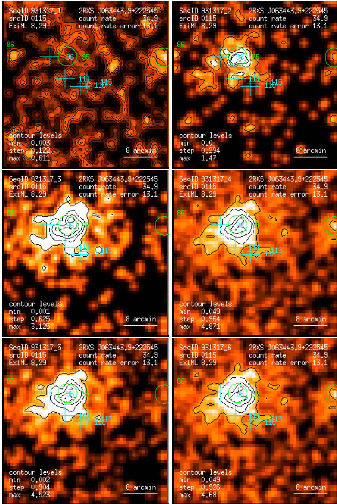
Figure 115: RASS 931317: detection 0115: band rate images, Gaussian filter: (1) PSPC channels 11 – 41, (2) 52 – 90, (3) 91 – 201, (4) 11 – 235, (5) 52 – 201, (6) 11 – 201. Broad band rates in counts/ks. Band rate contour levels in counts/ks/arcmin 2 .
