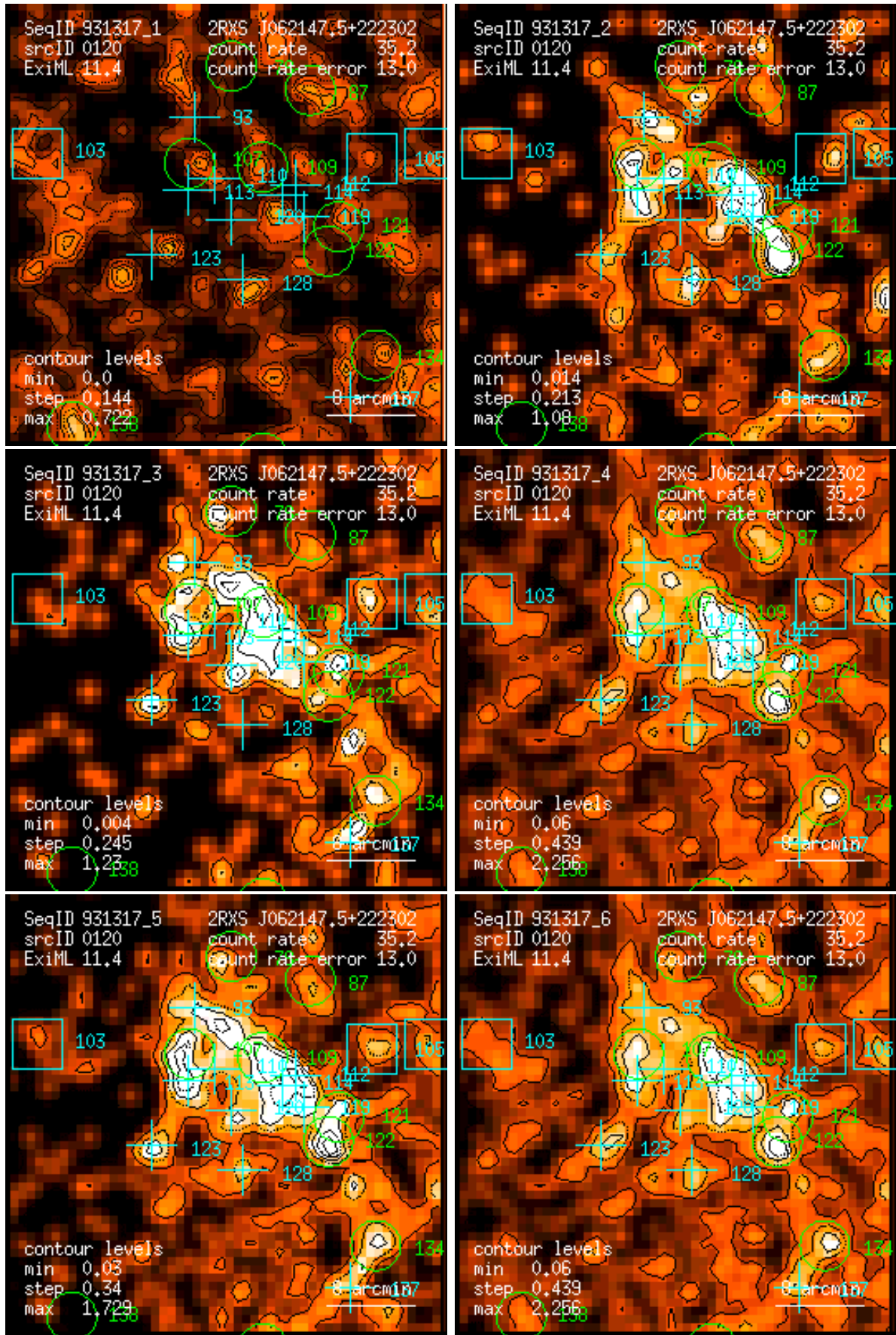
Figure 120: RASS 931317: detection 0120: band rate images, Gaussian filter: (1) PSPC channels 11 – 41, (2) 52 – 90, (3) 91 – 201, (4) 11 – 235, (5) 52 – 201, (6) 11 – 201. Broad band rates in counts/ks. Band rate contour levels in counts/ks/arcmin 2 .
