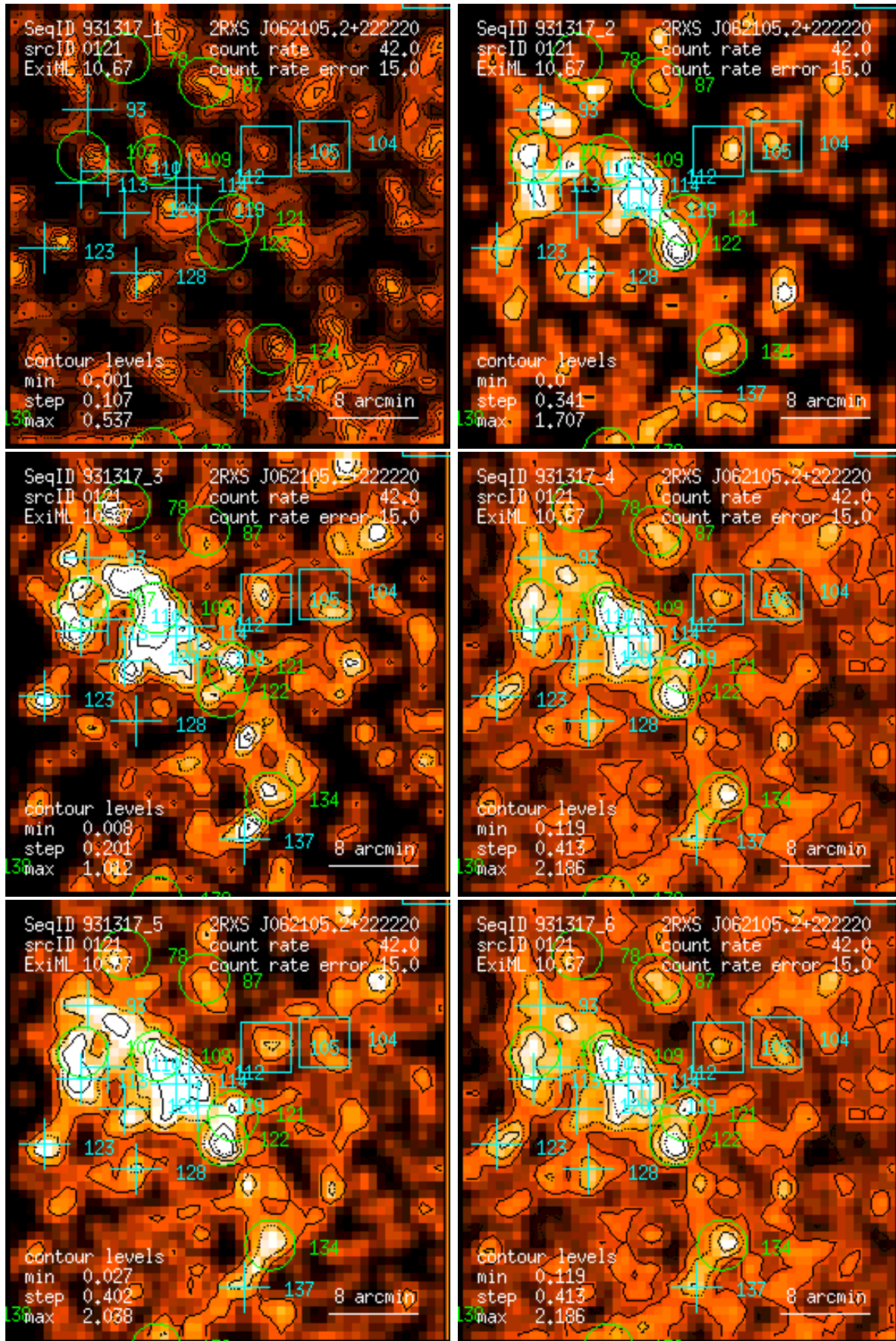
Figure 121: RASS 931317: detection 0121: band rate images, Gaussian filter: (1) PSPC channels 11 – 41, (2) 52 – 90, (3) 91 – 201, (4) 11 – 235, (5) 52 – 201, (6) 11 – 201. Broad band rates in counts/ks. Band rate contour levels in counts/ks/arcmin 2 .
