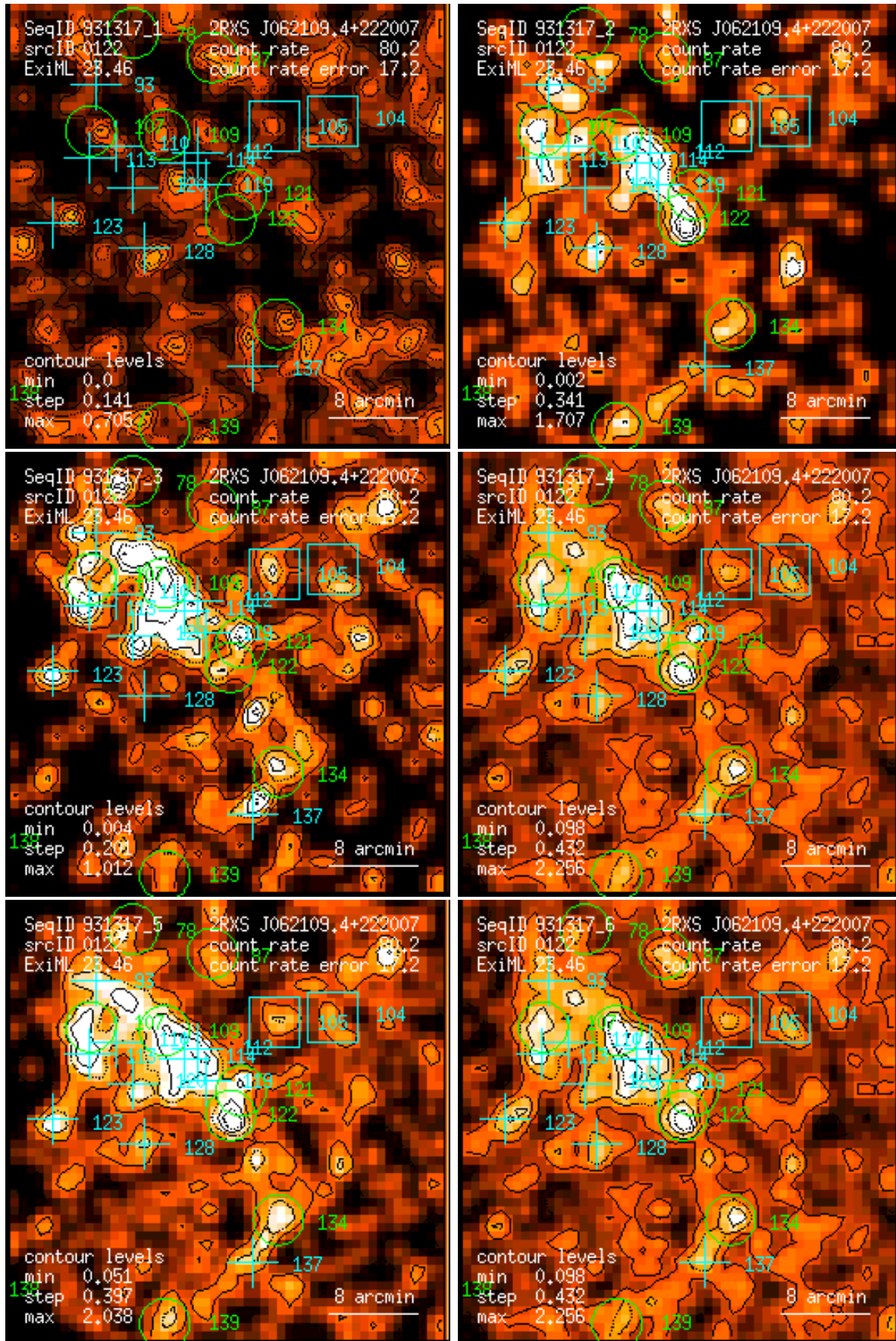
Figure 122: RASS 931317: detection 0122: band rate images, Gaussian filter: (1) PSPC channels 11 – 41, (2) 52 – 90, (3) 91 – 201, (4) 11 – 235, (5) 52 – 201, (6) 11 – 201. Broad band rates in counts/ks. Band rate contour levels in counts/ks/arcmin 2 .
