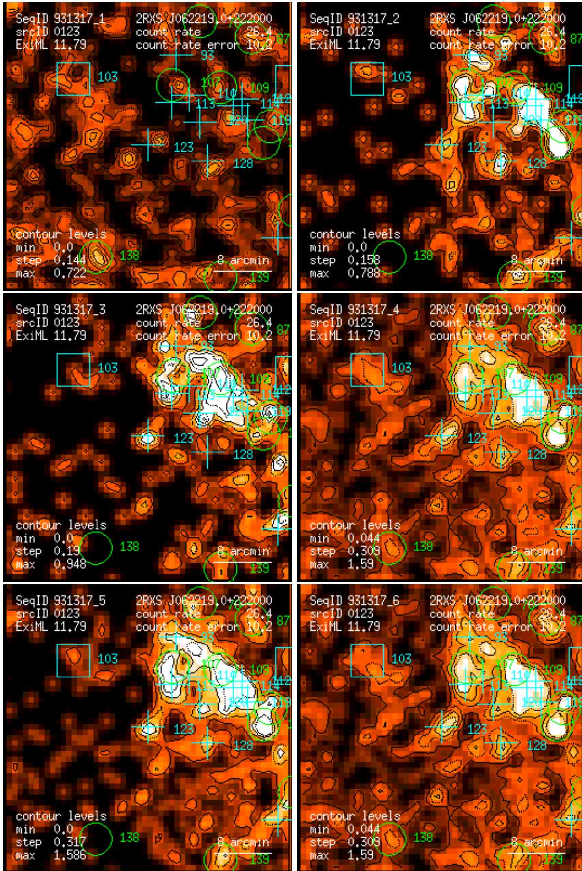
Figure 123: RASS 931317: detection 0123: band rate images, Gaussian filter: (1) PSPC channels 11 – 41, (2) 52 – 90, (3) 91 – 201, (4) 11 – 235, (5) 52 – 201, (6) 11 – 201. Broad band rates in counts/ks. Band rate contour levels in counts/ks/arcmin 2 .
