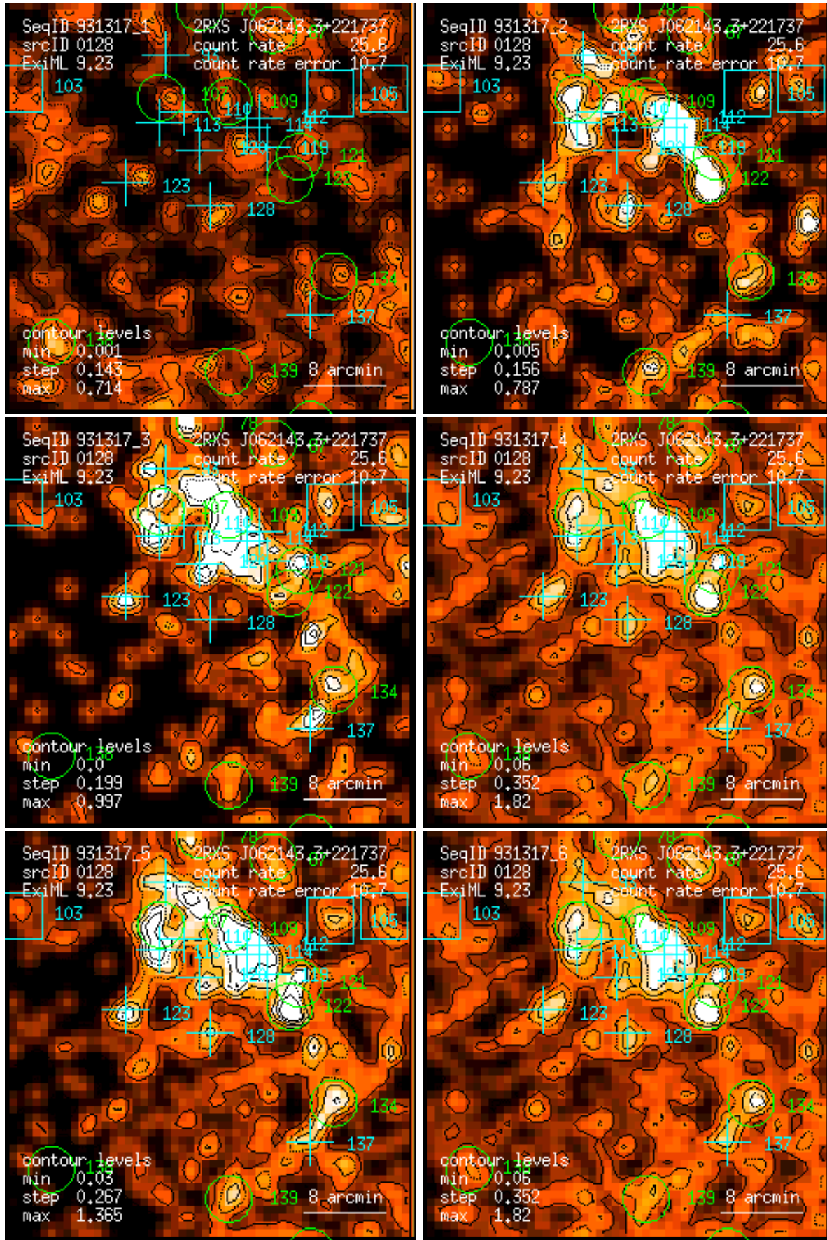
Figure 128: RASS 931317: detection 0128: band rate images, Gaussian filter: (1) PSPC channels 11 – 41, (2) 52 – 90, (3) 91 – 201, (4) 11 – 235, (5) 52 – 201, (6) 11 – 201. Broad band rates in counts/ks. Band rate contour levels in counts/ks/arcmin 2 .
