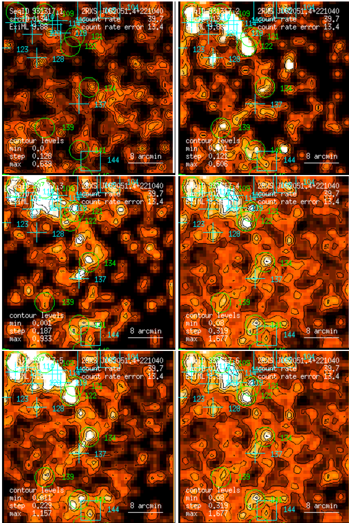
Figure 134: RASS 931317: detection 0134: band rate images, Gaussian filter: (1) PSPC channels 11 – 41, (2) 52 – 90, (3) 91 – 201, (4) 11 – 235, (5) 52 – 201, (6) 11 – 201. Broad band rates in counts/ks. Band rate contour levels in counts/ks/arcmin 2 .
