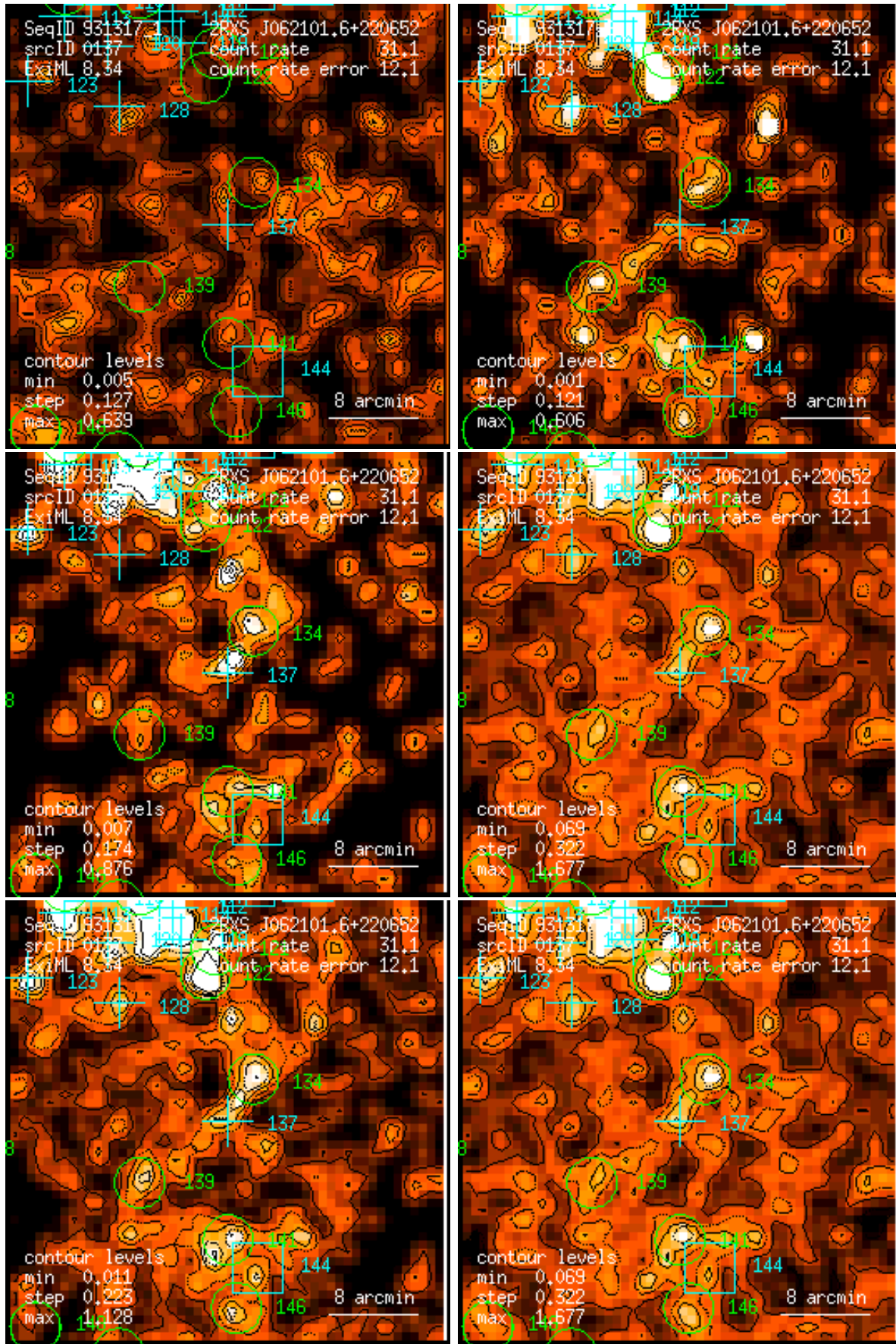
Figure 137: RASS 931317: detection 0137: band rate images, Gaussian filter: (1) PSPC channels 11 – 41, (2) 52 – 90, (3) 91 – 201, (4) 11 – 235, (5) 52 – 201, (6) 11 – 201. Broad band rates in counts/ks. Band rate contour levels in counts/ks/arcmin 2 .
