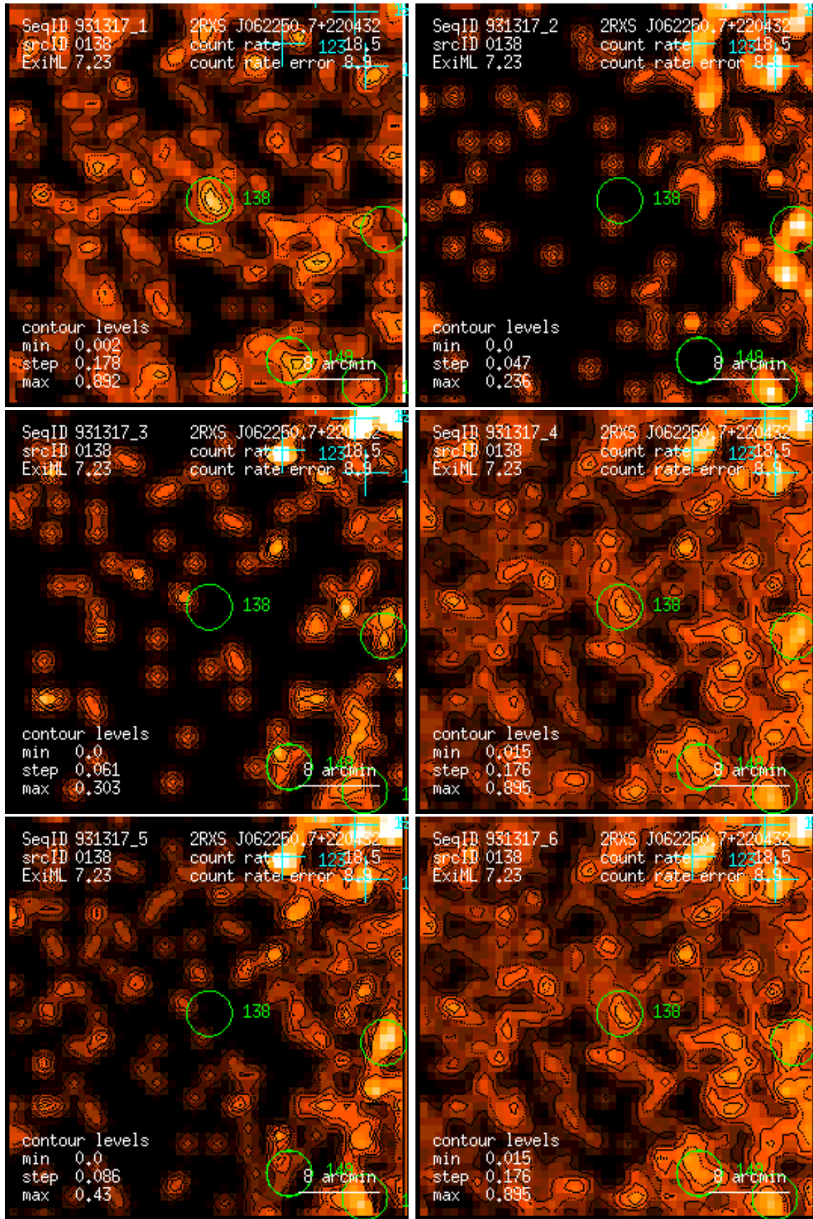
Figure 138: RASS 931317: detection 0138: band rate images, Gaussian filter: (1) PSPC channels 11 – 41, (2) 52 – 90, (3) 91 – 201, (4) 11 – 235, (5) 52 – 201, (6) 11 – 201. Broad band rates in counts/ks. Band rate contour levels in counts/ks/arcmin 2 .
