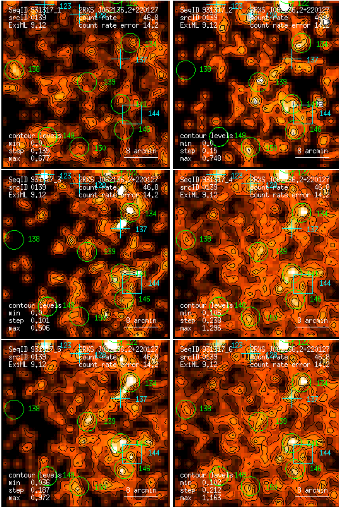
Figure 139: RASS 931317: detection 0139: band rate images, Gaussian filter: (1) PSPC channels 11 – 41, (2) 52 – 90, (3) 91 – 201, (4) 11 – 235, (5) 52 – 201, (6) 11 – 201. Broad band rates in counts/ks. Band rate contour levels in counts/ks/arcmin 2 .
