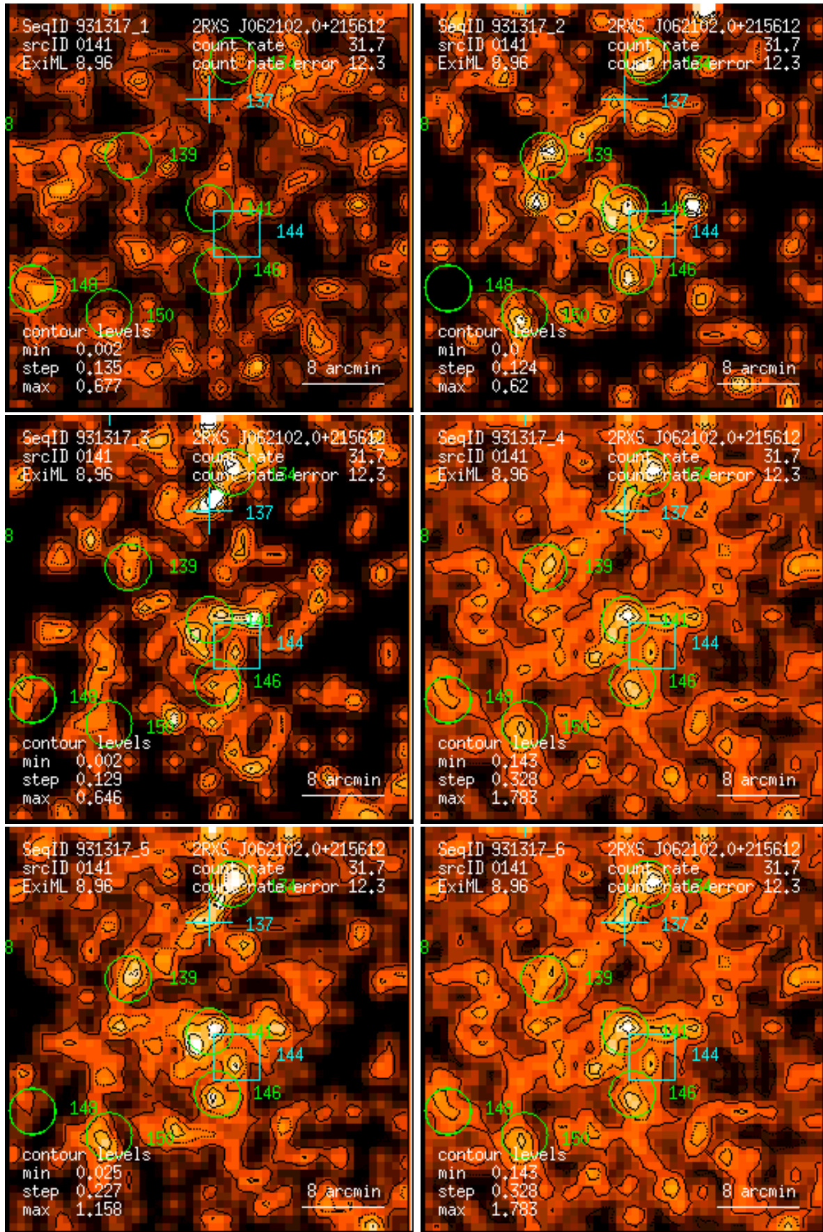
Figure 141: RASS 931317: detection 0141: band rate images, Gaussian filter: (1) PSPC channels 11 – 41, (2) 52 – 90, (3) 91 – 201, (4) 11 – 235, (5) 52 – 201, (6) 11 – 201. Broad band rates in counts/ks. Band rate contour levels in counts/ks/arcmin 2 .
