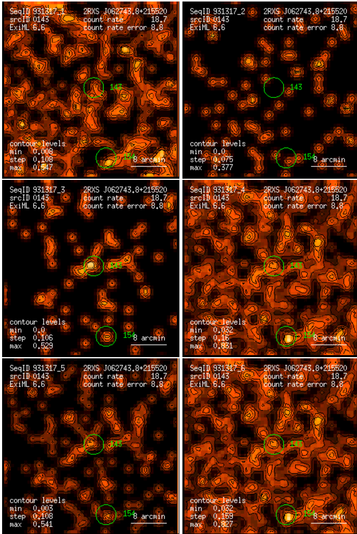
Figure 143: RASS 931317: detection 0143: band rate images, Gaussian filter: (1) PSPC channels 11 – 41, (2) 52 – 90, (3) 91 – 201, (4) 11 – 235, (5) 52 – 201, (6) 11 – 201. Broad band rates in counts/ks. Band rate contour levels in counts/ks/arcmin 2 .
