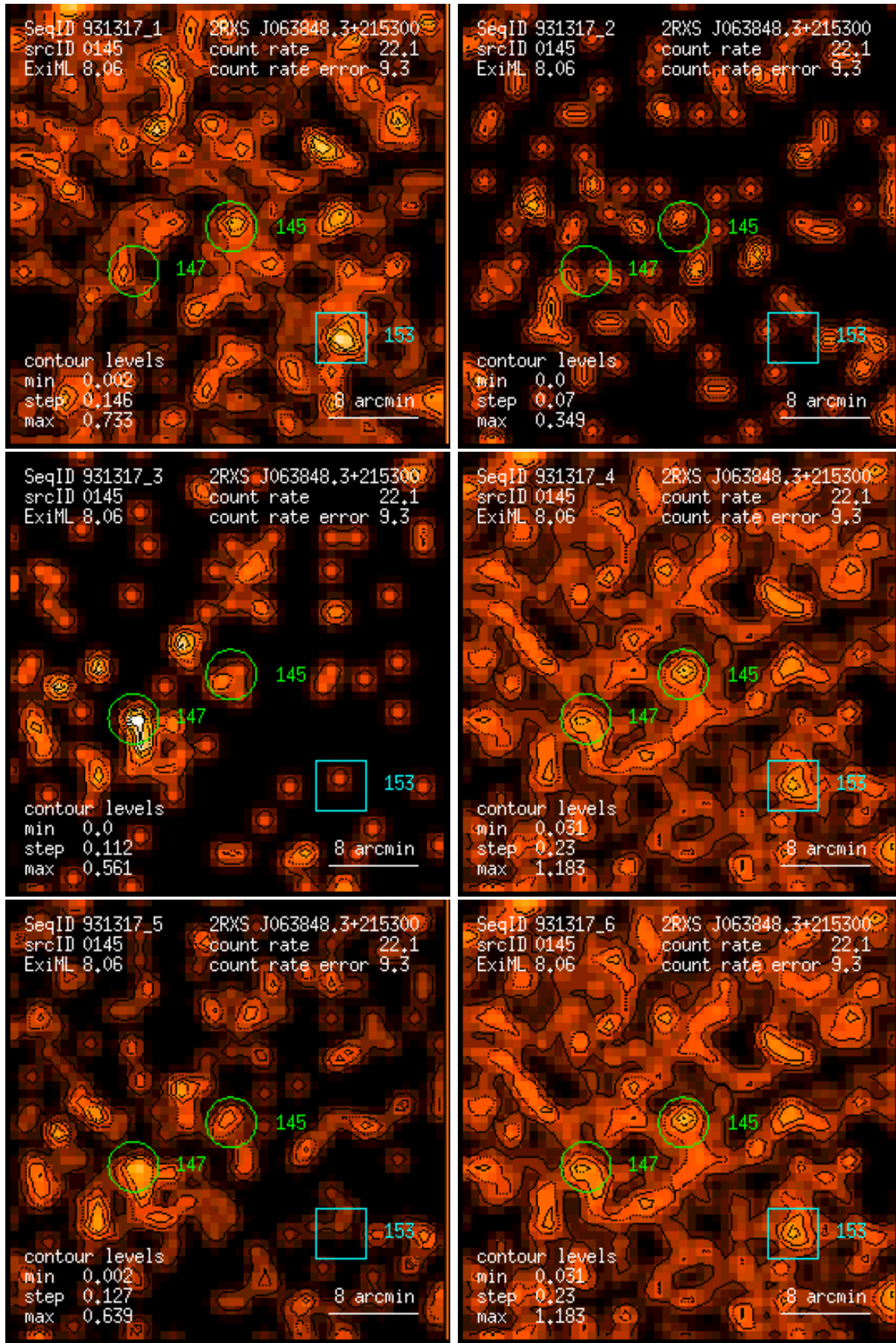
Figure 145: RASS 931317: detection 0145: band rate images, Gaussian filter: (1) PSPC channels 11 – 41, (2) 52 – 90, (3) 91 – 201, (4) 11 – 235, (5) 52 – 201, (6) 11 – 201. Broad band rates in counts/ks. Band rate contour levels in counts/ks/arcmin 2 .
