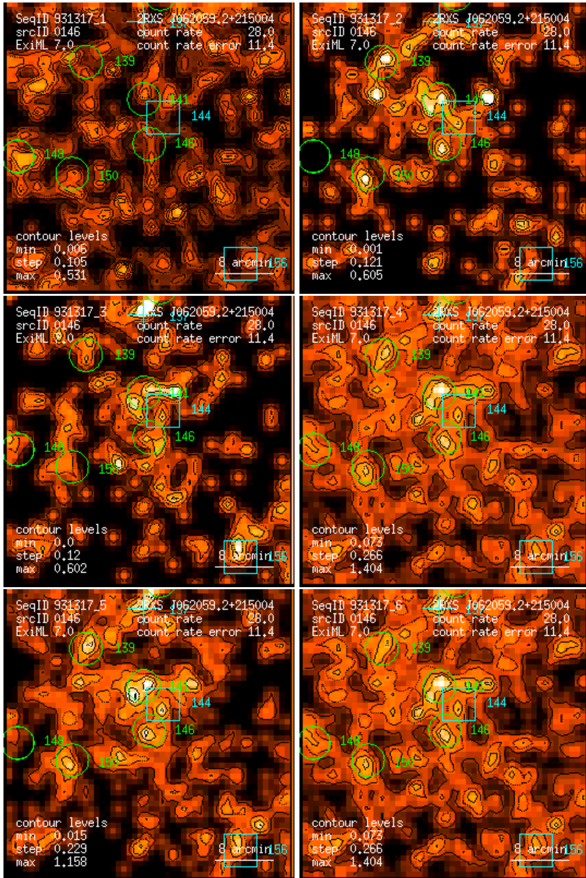
Figure 146: RASS 931317: detection 0146: band rate images, Gaussian filter: (1) PSPC channels 11 – 41, (2) 52 – 90, (3) 91 – 201, (4) 11 – 235, (5) 52 – 201, (6) 11 – 201. Broad band rates in counts/ks. Band rate contour levels in counts/ks/arcmin 2 .
