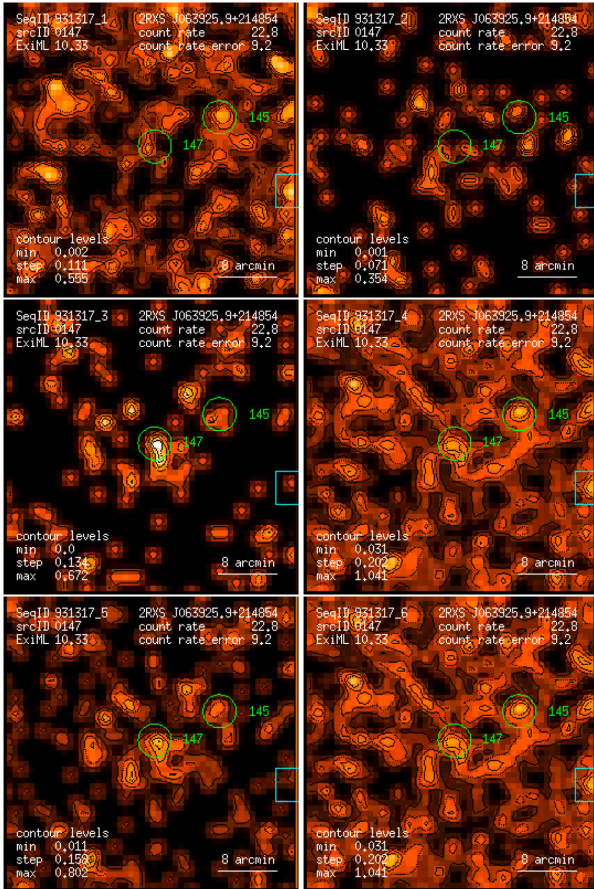
Figure 147: RASS 931317: detection 0147: band rate images, Gaussian filter: (1) PSPC channels 11 – 41, (2) 52 – 90, (3) 91 – 201, (4) 11 – 235, (5) 52 – 201, (6) 11 – 201. Broad band rates in counts/ks. Band rate contour levels in counts/ks/arcmin 2 .
