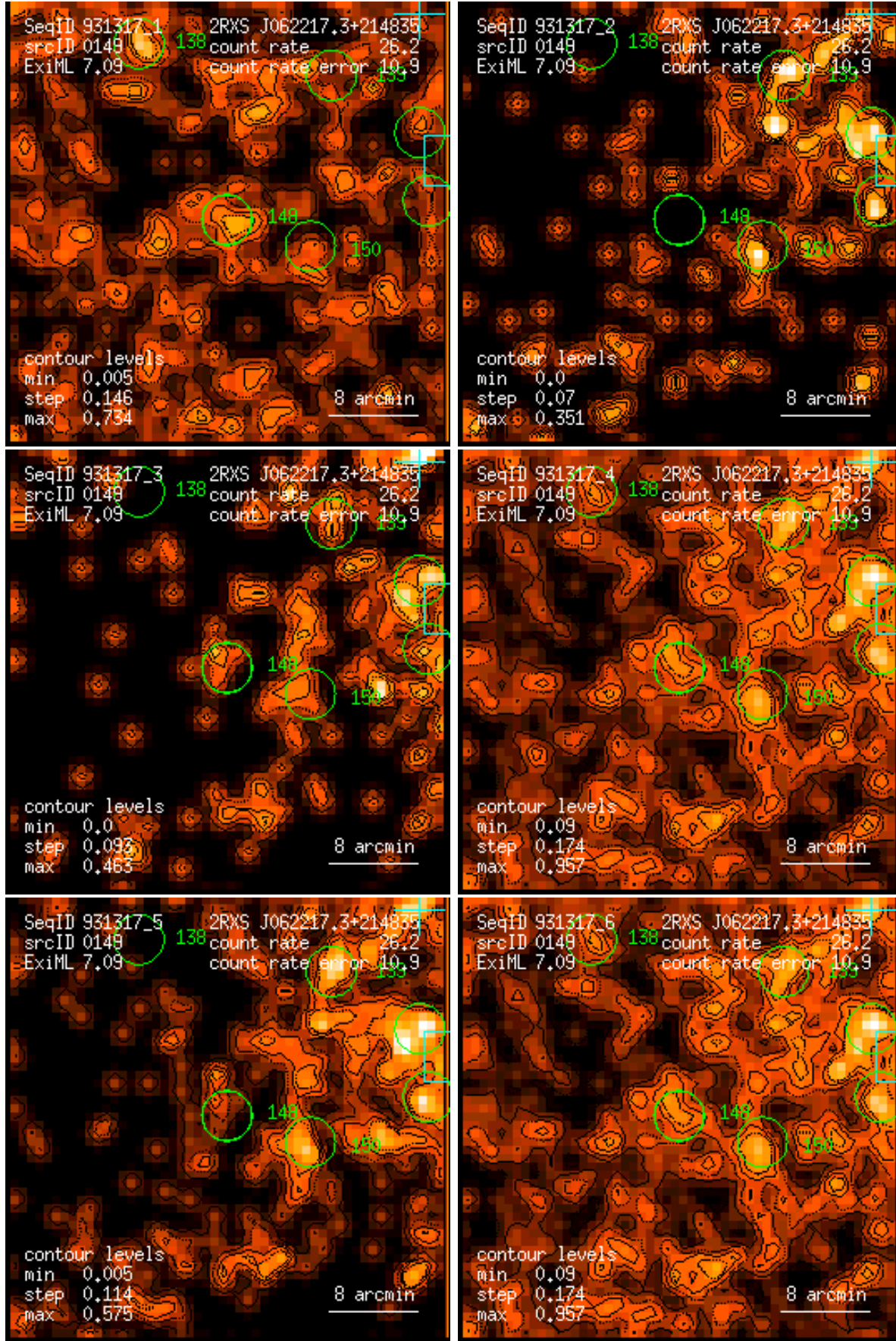
Figure 149: RASS 931317: detection 0149: band rate images, Gaussian filter: (1) PSPC channels 11 – 41, (2) 52 – 90, (3) 91 – 201, (4) 11 – 235, (5) 52 – 201, (6) 11 – 201. Broad band rates in counts/ks. Band rate contour levels in counts/ks/arcmin 2 .
